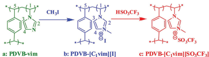
Fig. 13 Scheme for the synthesis of PDVB- [\text{C}_1\text{vim}][\text{SO}_3\text{CF}_3] from PDVB-vim via post-quaternization of the skeleton of the organic skeleton network followed by an anion exchange process. Reprinted with permission from ref. 41. Copyright 2012 American Chemical Society.
