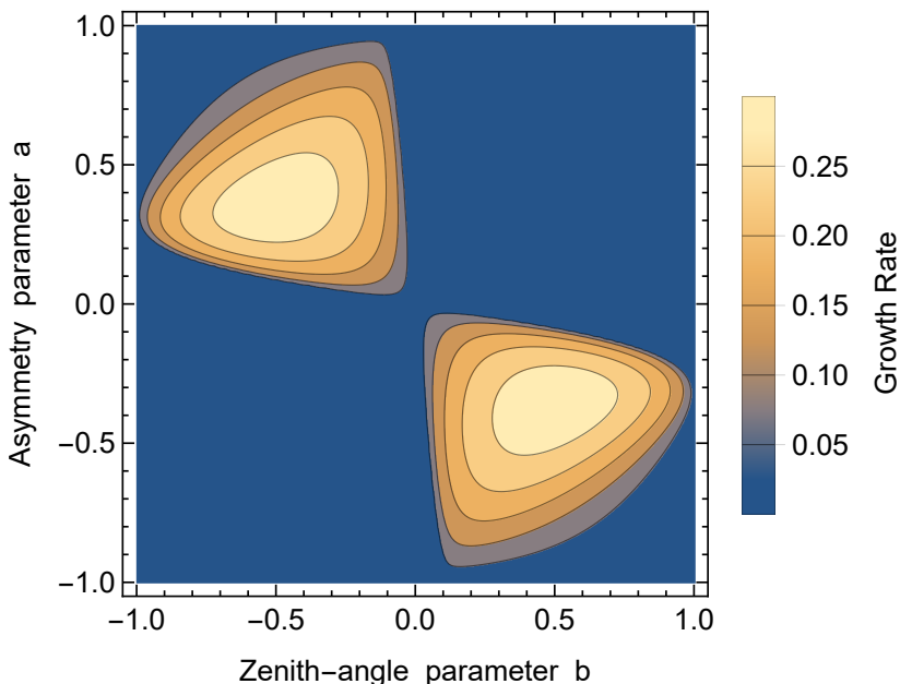
Figure 5. Growth rate in units of \mu for the axial-symmetry breaking solution of the two-bulb supernova model without matter. The normalized \nu_e density is 1 + a , for \bar{\nu}_e it is 1 - a . The \nu_e zenith-angle distribution is nonzero on the range 0 < u < 1 + b and on 0 < u < 1 - b for \bar{\nu}_e . The results show no instability in the SN motivated parameters ( a > 0 and b > 0 ), i.e., the first quadrant.
