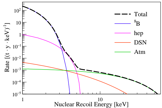
Figure 10. Event rate from coherent neutrino-nucleus scattering in xenon, in the energy region of interest for WIMP search: solar ( {}^8\text{B} and hep ), diffuse supernova (DSN) and atmospheric neutrinos (Atm).
