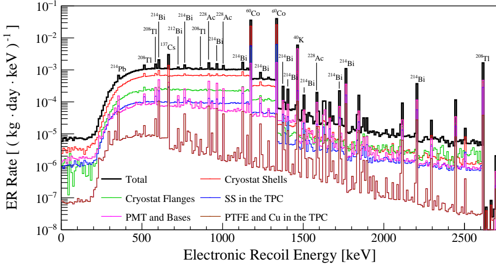
Figure 2. Energy spectrum in 1 t FV of the total ER background from the detector materials (black), and the separate contributions from the various components (colors).
