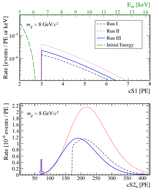
FIG. 6. Expected absolute rate in cS1 (top) and cS2 b (bottom) of an 8 GeV/c 2 WIMP SI signal and a cross section of 1 \times 10^{-44} cm 2 for each science run. The initial energy spectrum in keV nr is shown (green long-dashed). The average LCE = 1 is shown for example, resulting in the hard cut at S1 = cS1 = 3 PE. The S2 thresholds for runs II and III are indicated by the vertical arrows. The differences in the spectra are due to varying exposures, S2 threshold, and acceptances.
