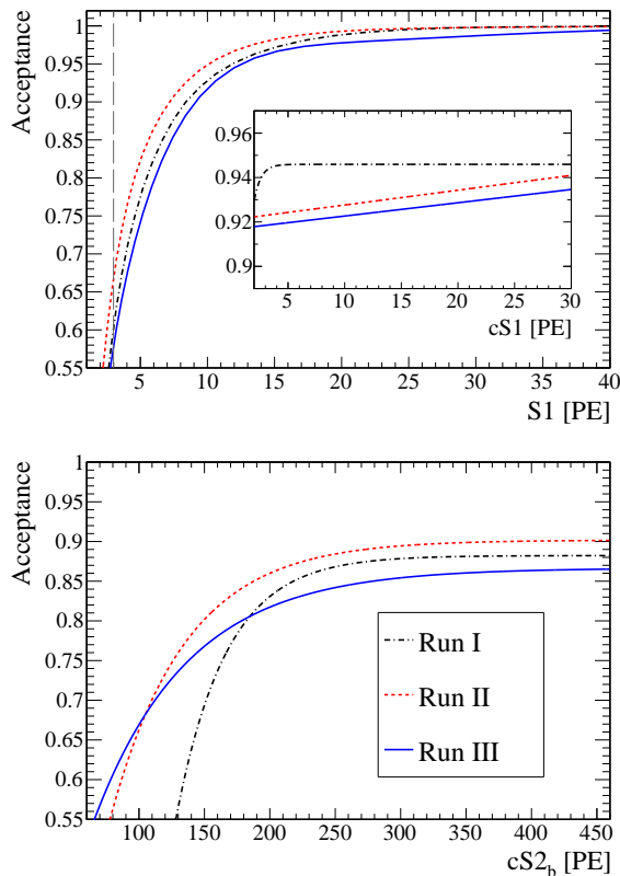
FIG. 4. The S1 coincidence cut acceptance combined with the noise misidentification acceptance (top), and the cumulative acceptance of the rest of the cS1-based cuts (top-inset) and cS2-based cuts (bottom), for each science run. The acceptance in cS2 is constant above 450 pe.
