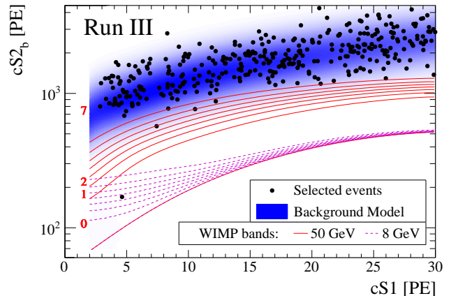
FIG. 5. Example bands for 8 GeV/ c^2 (purple dashed lines) and 50 GeV/ c^2 (red solid lines with numbered labels) WIMP mass SI signal models. The upper bound of the top-most band is beyond the vertical range. The shape of the background model is shown with a shaded (blue) linear z-axis scale. The run III science data are overlaid for reference.
