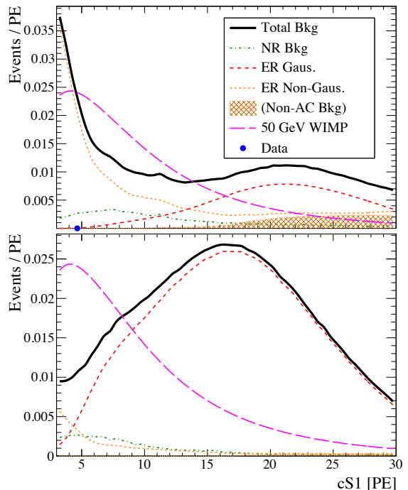
FIG. 8. Expected event rates for PL band 0 (top) and 2 (bottom) from Fig. 5 for a 50 \text{ GeV}/c^2 WIMP and an assumed SI cross-section of \sigma_{SI} = 10^{-45} \text{ cm}^2 (long-dashed magenta line). The contribution from various background components described in the text (non-solid colored lines) are shown together with their sum (solid black line). The non-AC component of the total non-Gaussian ER background is shown (diagonal line filled area). The run III models are shown for example and the cS1 of the ROI event is shown on the horizontal axis (blue point).
