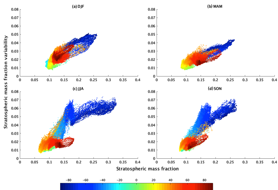
Figure 4: Scatterplots showing the \text{CH}_4 stratospheric column mass fraction ( f_{\text{str}} ) against \text{CH}_4 stratospheric column mass fraction variability ( \sigma_{\text{str}} ) for (a) December-February, (b) March-May, (c) June-August and (d) September-November months of 2010. The colour shading indicates different latitude bands.
