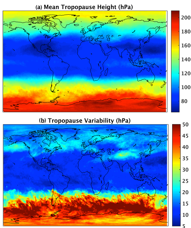
Figure 3: (a) Mean tropopause height (in hPa) and (b) variability (standard deviation) of tropopause height (in hPa) from the C-IFS model fields for June - August 2010.
