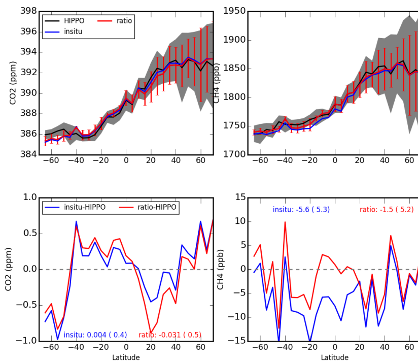
585 Figure A2: (Top) HIPPO-3 (Wofsy et al., 2011), May 2010, and a posteriori model partial columns of (left) \text{CO}_2 and (right) \text{CH}_4 as a function of latitude over the Pacific Ocean, and (bottom) the differences between the observations and the in situ and ratio inversions. The mean biases (standard deviations) between the model and data are shown in set of lower panels. Data and model values are binned into 5^\circ mass-weighted latitude boxes.
