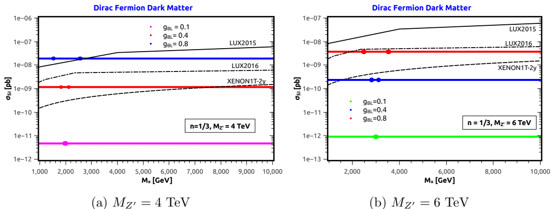
Figure 5: Dirac Fermion. Spin-independent dark matter-nucleon scattering cross section as a function of the dark matter mass with n = 1/3 and M_{Z'} = 4, 6 \text{ TeV} for different gauge couplings, g_{BL} = 0.1, 0.4, 0.8 . The current limit from LUX-2015 (solid line) [97], preliminary limit from LUX-2016 (dotted-dashed)[98] and the one projected from XENON1T (dashed line) for two years of data taking [19] are also shown.
