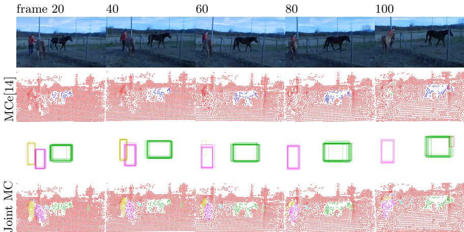
Fig. 5. Comparison of the proposed Joint Multicut model and the multicut on trajectories (MCE) [14] on the horses06 sequence of FBMS59.
