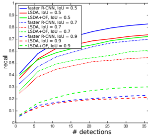
(a) The detection performance of LSDA [45] and faster R-CNN [46]. We compare the recall for three different IoU thresholds 0.9, 0.7, and 0.5.
