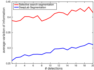
(b) The Variation of Information for the proposed object masks over the number of detections (lower is better).
