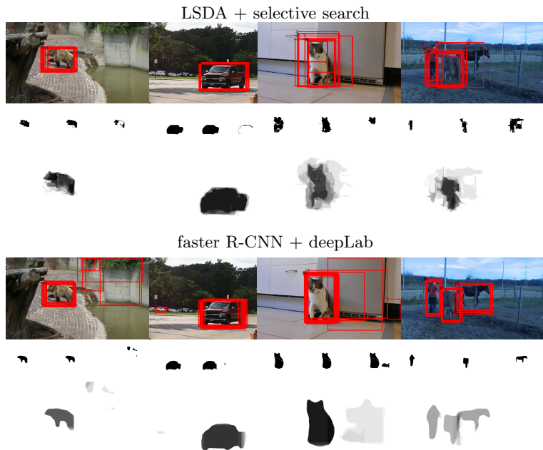
Fig. 2. Examples of the object detections and according segmentations. Top: LSDA detections on images from FBMS59 sequences [11]. The first row shows the best 20 detections. The second row shows three exemplary selective search proposals and third row visualizes the average segmentation of all proposals. Bottom: The corresponding faster R-CNN detections. The first row shows the best 20 detections with a minimum detection score of 0.2. The second row shows three exemplary segmentations from deepLab [51,52] on these detections and third row visualizes the average segmentation.
