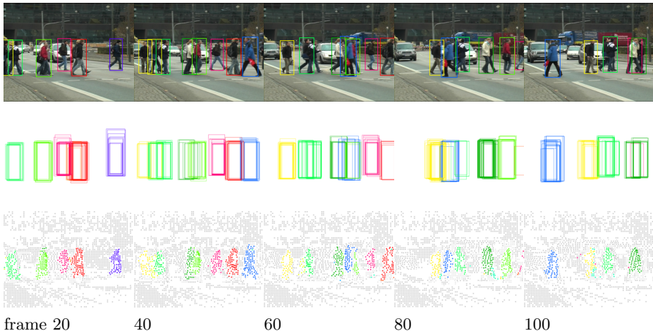
Fig. 7. Results of the proposed Joint Multicut model on the TUD-crossing sequence.
