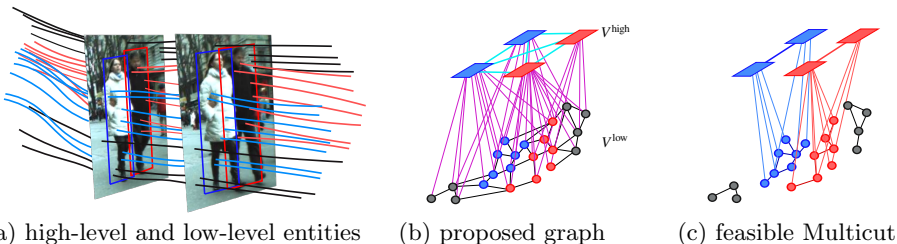
Fig. 1. (a) While pedestrian detections, here drawn as bounding boxes, represent frame-wise high-level information, point trajectories computed on the same sequence represent spatio-temporal low-level cues. Both can be represented as vertices in a joint graphical model (b). The optimal decomposition of this graph into connected components yields both a motion trajectory segmentation of the sequence as well as the tracking of moving objects represented by the detections (c).
