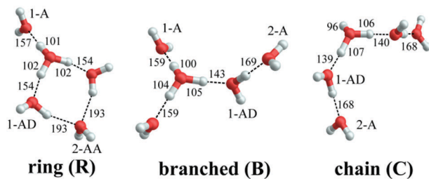
Fig. 1 B3LYP-D3/aug-cc-pVTZ minimum-energy structures of the three constitutional isomers discussed in the text. Intramolecular hydronium ion O–H and intermolecular hydrogen bond lengths are reported in pm. Water molecules are classified according to their location in the first (1) or second (2) hydration shell of \text{H}_3\text{O}^+ , and their function as hydrogen bond acceptor (A) or donor (D).
