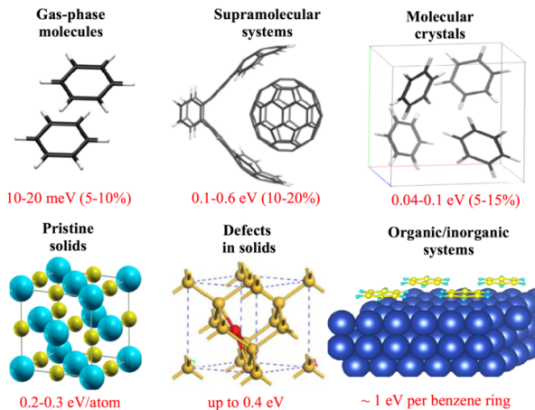
FIG. 3 (Color online) Various types of materials with calculated cohesion energies and errors as compared to available reference data. The top row of values shows typical errors of atomistic vdW methods compared to benchmark binding energies, while the bottom row of values shows contributions of the vdW energy to the binding energy of the corresponding materials.
