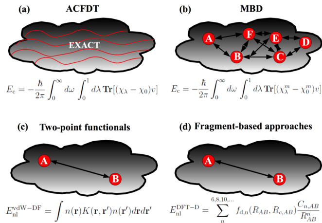
FIG. 2 (Color online) Schematic representation of first principles methods for the (a) exact formulation of the electronic correlation energy E_c from the adiabatic connection fluctuation-dissipation theorem; (b) formulation based on coupled dipolar fluctuations, such as the many-body dispersion (MBD) methods (Ambrosetti et al. , 2014c; Tkatchenko et al. , 2012b); (c) E_c using two-point functionals obtained by approximating the non-homogeneous system with a homogeneous-like response; and (d) fragment-based correlation energy obtained from multipolar expansions.
