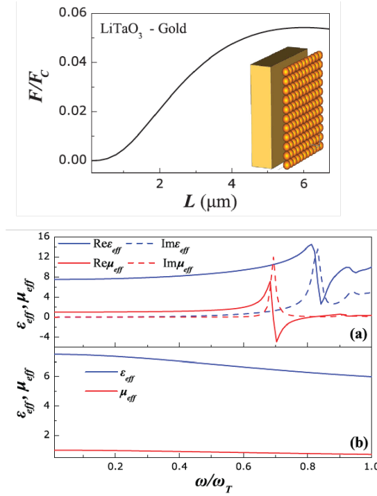
FIG. 10 (Color Online) Top: Normalized Casimir force as a function of separation between a gold semi-space and a 2D metasurface made of close-packed (lattice constant a = 11.24\mu\text{m} ) \text{LiTaO}_3 spheres of radius r = 5.62\mu\text{m} , calculated via scattering theory. The optical response of \text{LiTaO}_3 is described by a single-resonance Drude-Lorentz model, \epsilon(\omega) = \epsilon_\infty(1 + \frac{\omega_L^2 - \omega_T^2}{\omega_T^2 - \omega^2 - i\omega\gamma}) , where \epsilon_\infty = 13.4 , the transverse and longitudinal optical phonon frequencies are \omega_T = 26.7 \times 10^{12} rad/sec and \omega_L = 46.9 \times 10^{12} rad/sec, and the dissipation parameter is \gamma = 0.94 \times 10^{12} rad/sec. The gold Drude parameters are taken as \hbar\Omega_p = 3.71 eV and \Omega_p\gamma_p^{-1} = 20 . Bottom: effective permittivity and permeability of the close-packed \text{LiTaO}_3 spheres as a function of (a) real and (b) imaginary frequencies as calculated by the Maxwell-Garnett effective medium theory. Figures taken from (Yannopapas and Vitanov, 2009).
