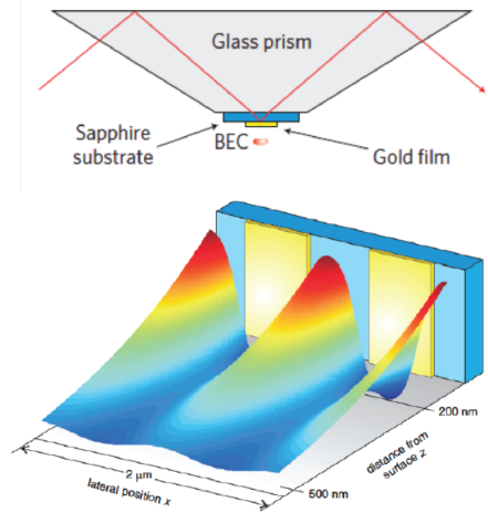
FIG. 12 (Color Online) Top: Schematic configuration to measure the Casimir-Polder potential probed by a Bose-Einstein condensate diffracted from a plasmonic nanostructured being excited by an external laser field in the Kretschmann configuration. Bottom: Atom-grating potential landscape arising from the combination of a repulsive evanescent-wave potential and the Casimir-Polder attraction. The external laser field has a power of P = 211 mW. The evanescent field from the grating modulates the repulsion, and the attractive Casimir-Polder potential is the strongest on top of the gold stripes. At a distance of 200 nm, the potential is laterally modulated with an amplitude of \Delta E/k_B = 14\mu\text{K} . Figures taken from (Bender et al. , 2014; Stehle et al. , 2011).
