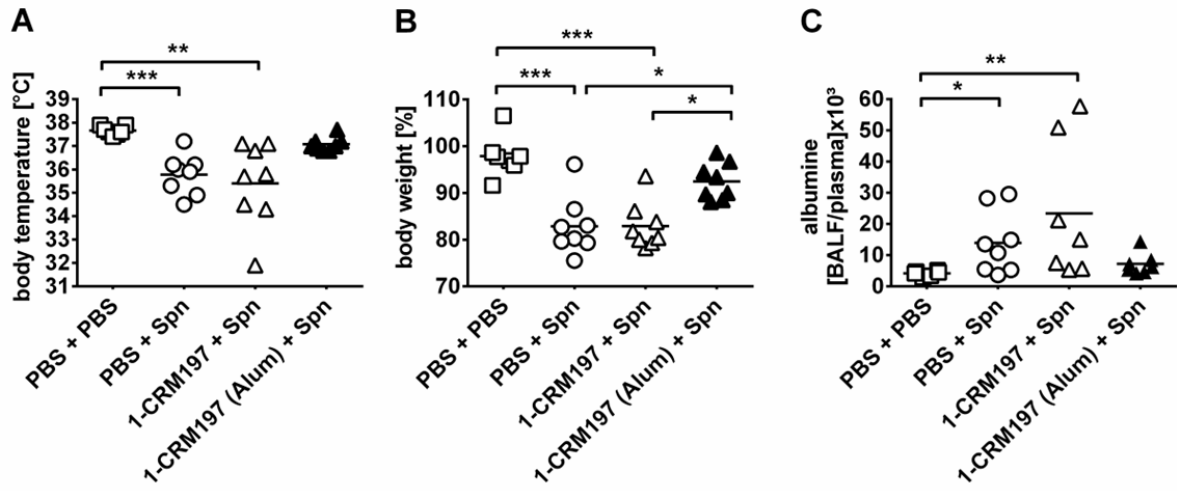
Figure 5. Effect of vaccination on pneumonia severity. After immunization on days 0, 14 and 28 mice were infected transnasally with 1 \times 10^6 cfu S. pneumoniae (Spn) or sham infected with PBS on day 35. (A) Body temperature (n=7-8), (B) body weight (n=7-8), and (C) lung permeability (n=6-8) were assessed 48 h after infection.
