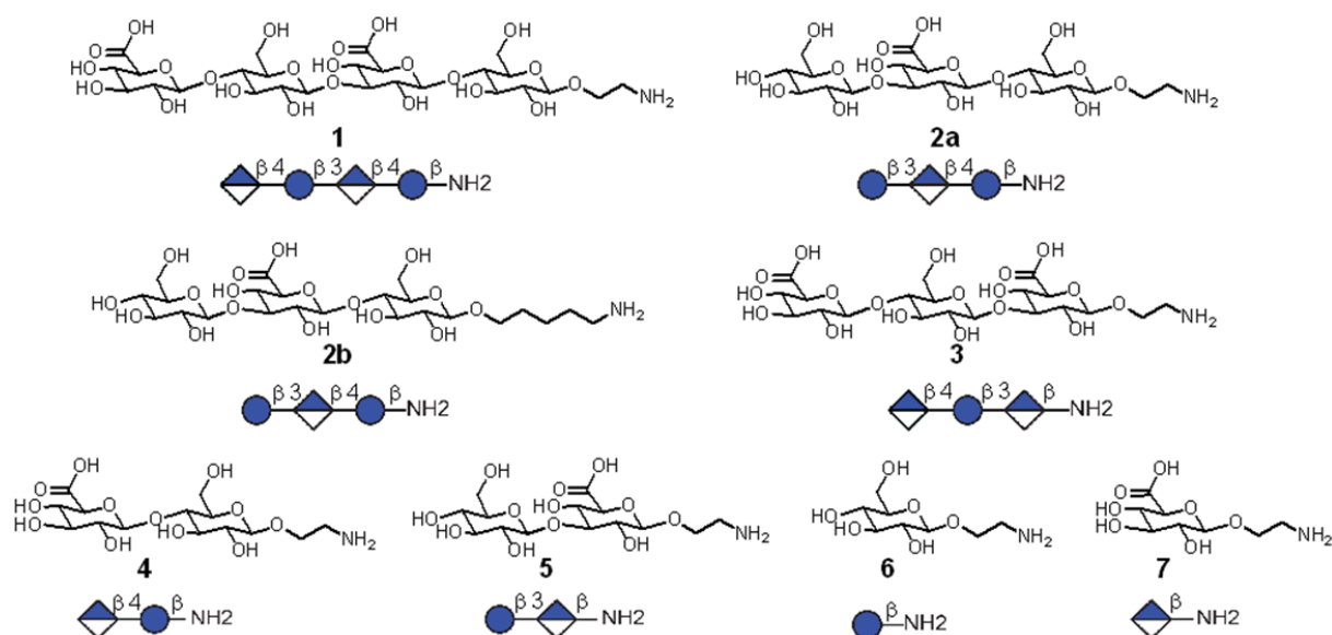
Figure 1: Synthetic ST3 glycans 1–7 based on the repeating unit of ST3-CPS.
