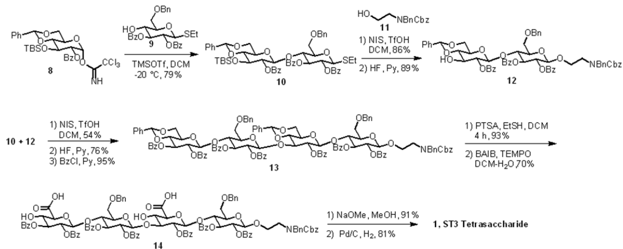
Scheme 1: Synthesis of ST3 tetrasaccharide 1
