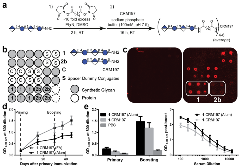
Figure 2: Glycan array analysis of protective murine mAbs raised against ST3-CPS. (A) Simplified printing pattern only showing bound compounds. Complete printing pattern is shown in Figure S1. (B) Representative glycan array fields showing binding pattern of mAbs 1E2 and 5F6. (C) Comparison of binding strengths of mAbs at 16 \mu g/mL represented by fluorescence intensities. Each bar is the mean of four spots with the error bar representing the standard error of mean (SEM). Significance levels were calculated by pairwise Bonferroni comparison after two-way analysis of variance (ANOVA). A glycan array analysis of human reference serum 007sp is shown in Figure S2.
