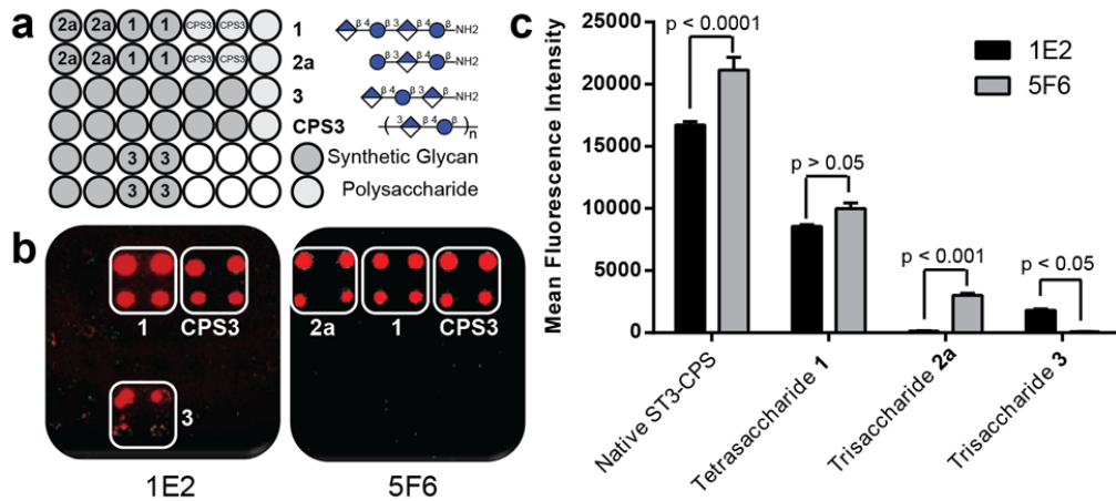
Figure 2: Glycan array analysis of protective murine mAbs raised against ST3-CPS. (A) Simplified printing pattern only showing bound compounds. Complete printing pattern is shown in Figure S1. (B) Representative glycan array fields showing binding pattern of mAbs 1E2 and 5F6. (C) Comparison of binding strengths of mAbs at 16 \mu g/mL represented by fluorescence intensities. Each bar is the mean of four spots with the error bar representing the standard error of mean (SEM). Significance levels were calculated by pairwise Bonferroni comparison after two-way analysis of variance (ANOVA). A glycan array analysis of human reference serum 007sp is shown in Figure S2.
