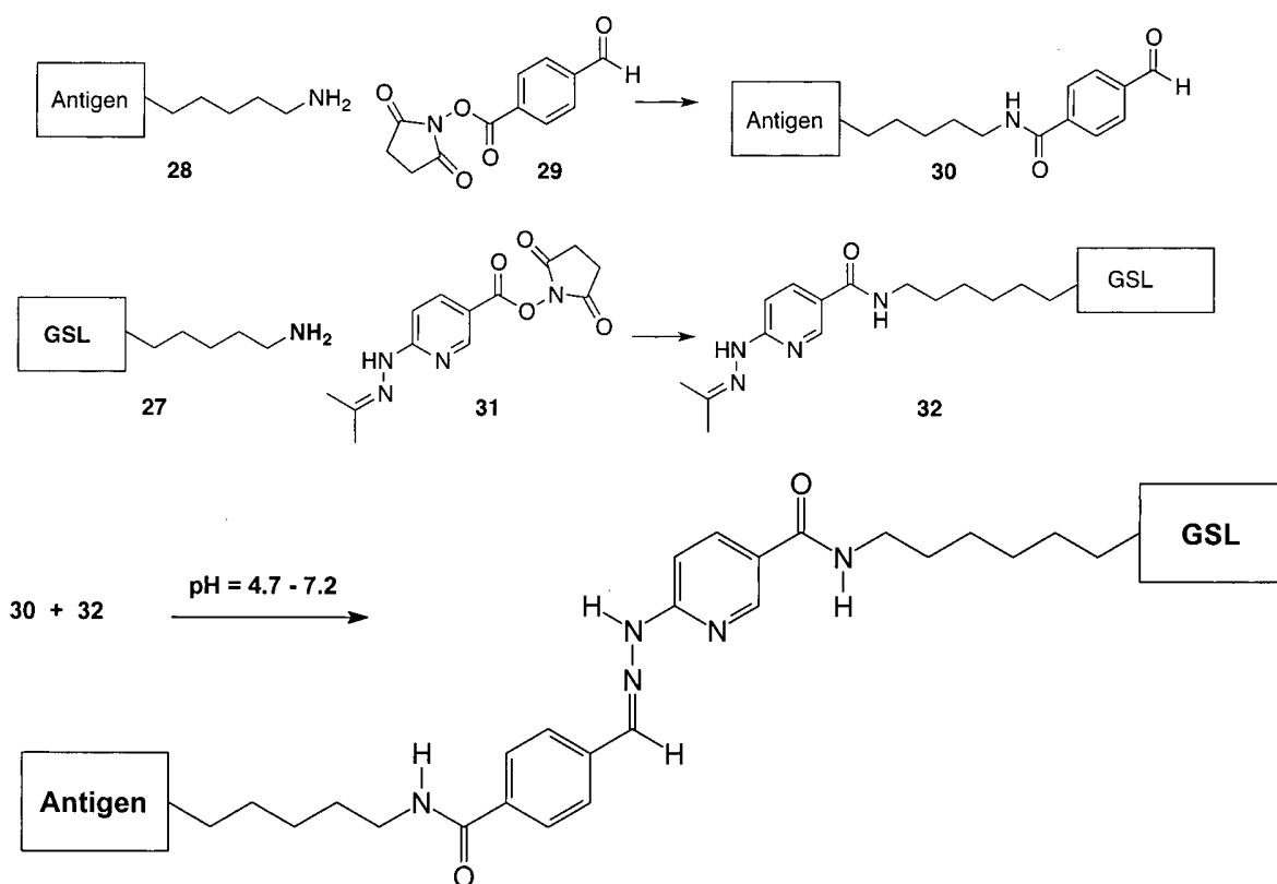
Scheme 5. Conjugation of amine linker-equipped antigen 28 with glycolipid 27 via hydrazone linkage.
