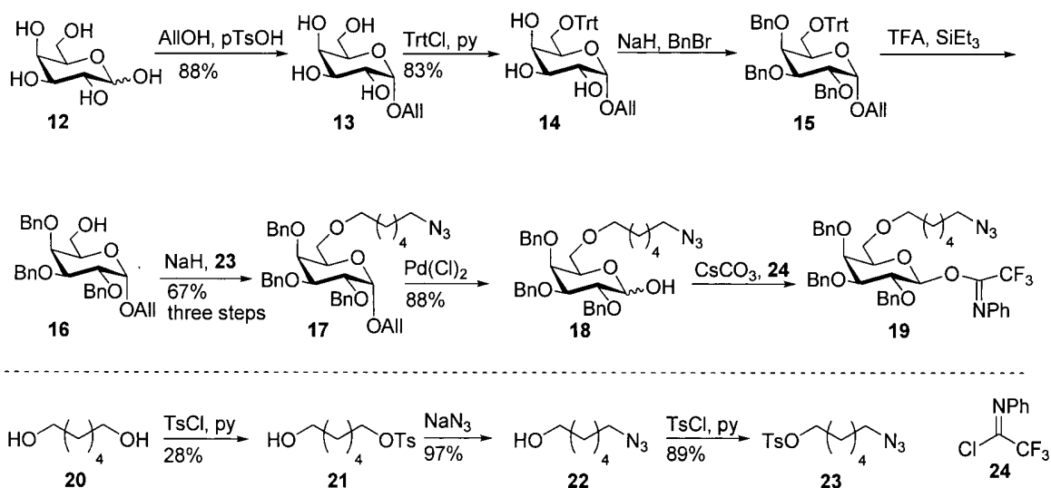
5 Scheme 2. Synthesis of galactosylating agent 19 .
