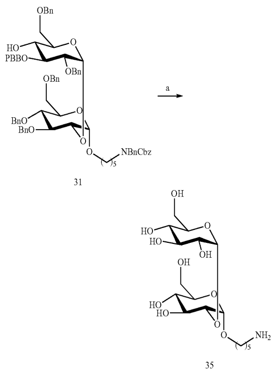
Scheme 10. Synthesis of 35.
