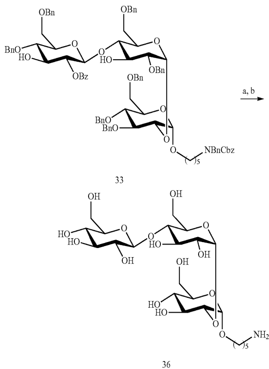
Scheme 11. Synthesis of 36.
