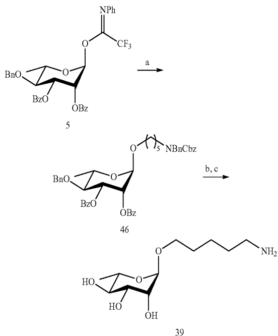
Scheme 14. Synthesis of 39.
