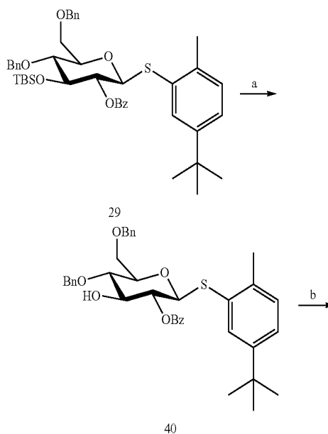
Scheme 12. Synthesis of 38.
