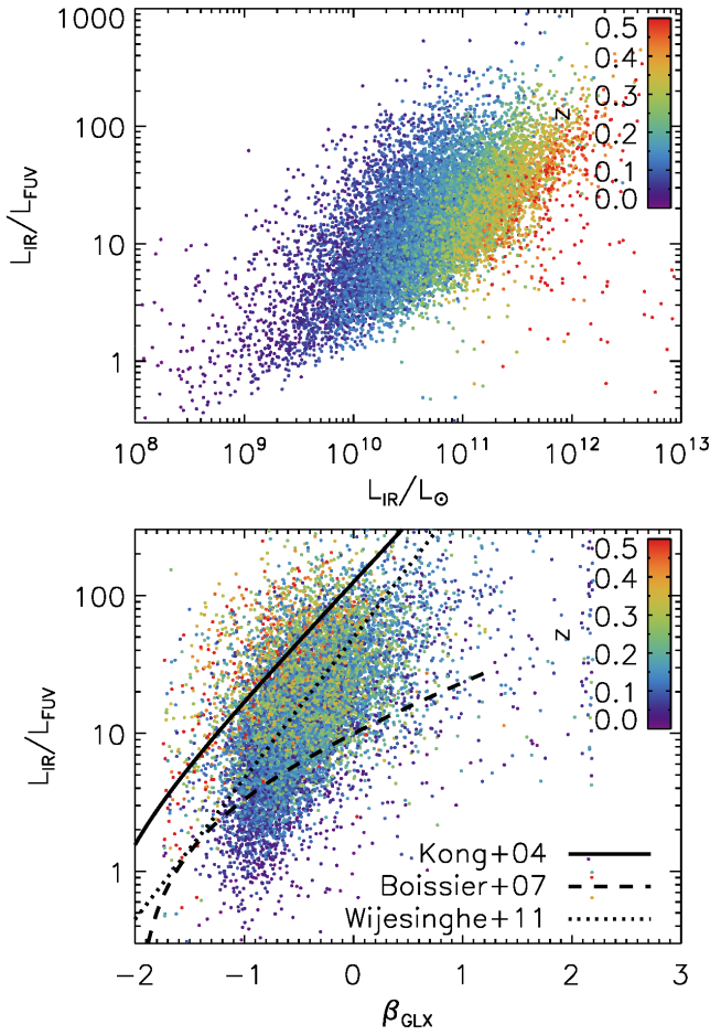
Figure 20. Ratio of rest-frame total IR luminosity to rest-frame FUV -band luminosity ( \nu L_{\nu} ) for H-ATLAS sources which have reliable IDs in GAMA and FUV detections from GALEX , as a function of L_{IR} (top) and \beta_{GLX} (bottom), where \beta_{GLX} = (\log f_{FUV} - \log f_{NUV}) / (\log \lambda_{FUV} - \log \lambda_{NUV}) as defined by Kong et al. (2004). Also shown on the lower panel are the best-fit relations for local starbursts (Kong et al. 2004), local late-type galaxies (Boissier et al. 2007), and galaxies selected from the H-ATLAS SDP+GAMA (Wijesinghe et al. 2011).
