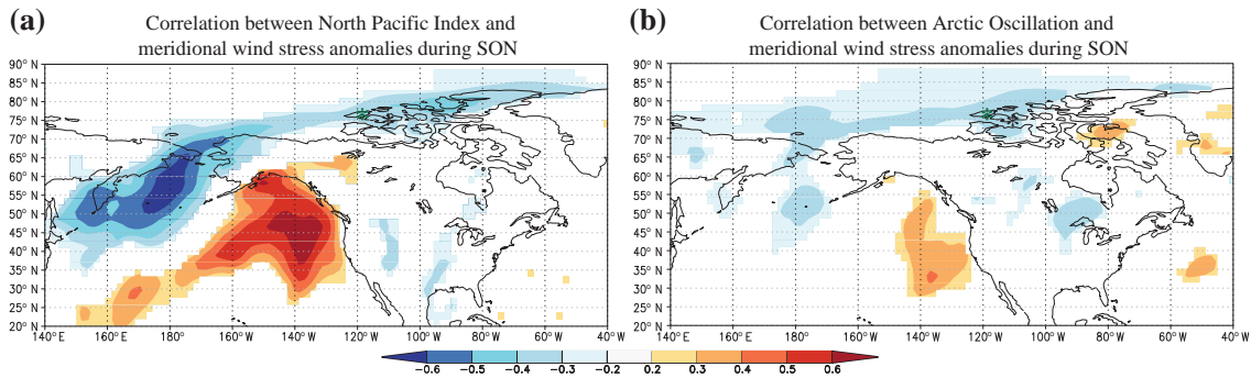
Figure 6. (a) Correlation between NPI (Trenberth and Hurrell, 1994) and meridional wind stress anomalies from 1950 to 2015. (b) Same as (a), but for correlation with Arctic Oscillation index (derived from NCEP/CPC). Note that the ERA-Interim yields similar results (not shown). Black and green asterisks denote Cape Bounty and Mould Bay weather stations respectively.
