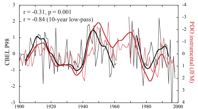
Figure 3. Instrumental PDO (NOAA) compared with grain size at Cape Bounty East Lake from 1900 to 2000 (best correlation is achieved when CBEL lags PDO by 1 year). Bold lines are 10-year low-pass filtered. A turbidite dated to 1971 CE eroded 7 years (Lapointe et al., 2012).
