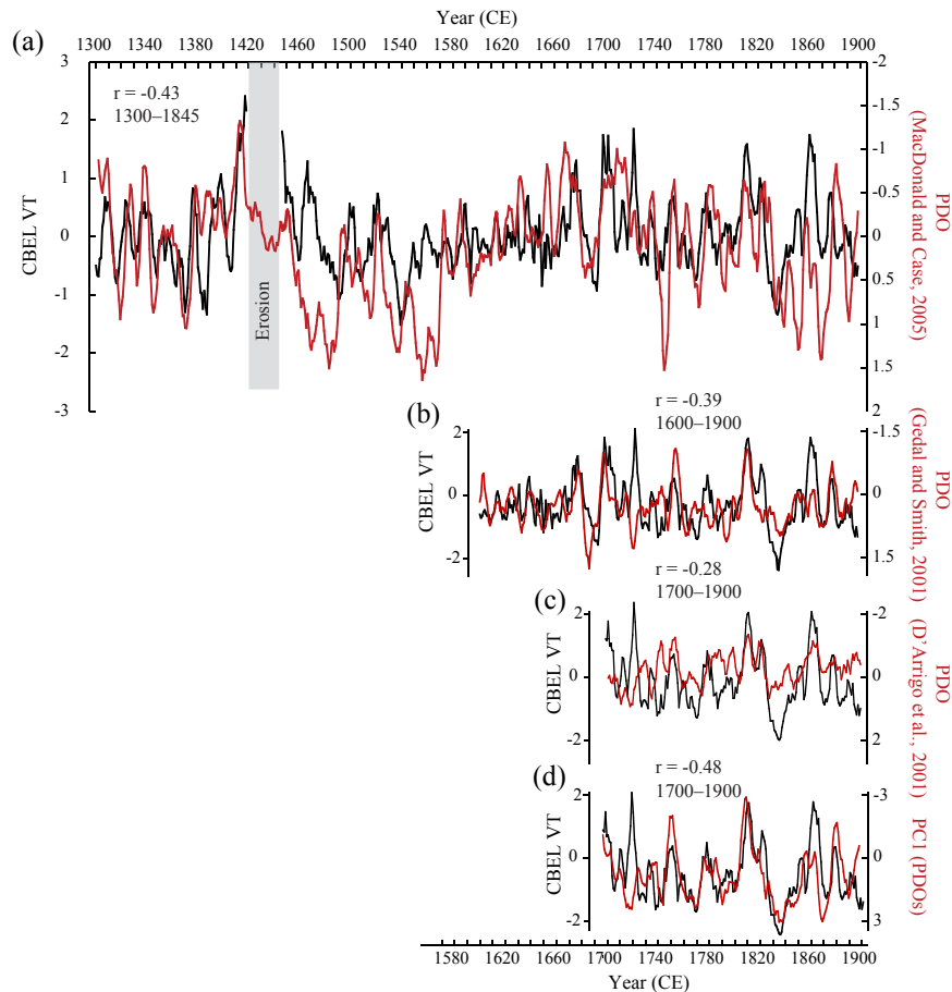
Figure 4. (a) Comparison between normalized Cape Bounty East Lake varve thickness and normalized PDO from MacDonal and Case (2005) (VT is shifted 18 years earlier). (b) Same as (a) but for the PDO from Gedalof and Smith (2001). (c) Same as (a) and (b) but using the PDO from D'Arrigo et al. (2001). (d) Same as (a), (b) and (c) but using the PC1 extracted from PCA analysis of the three PDOs. Time series are filtered by a 5-year running mean.
