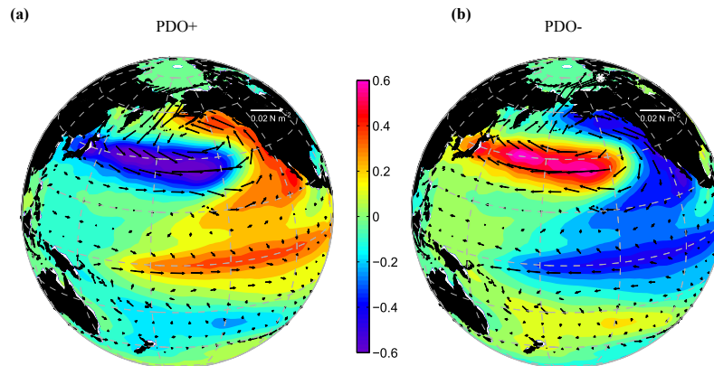
Figure 7. PDO modulation of winds and sea surface temperature in the Pacific (Zhang and Delworth, 2015). Regression of SST ( ^{\circ}\text{C} ) and surface wind stress ( \text{N m}^{-2} ) against the PDO index. Note the northward direction of the wind stress in the central northern part of the Pacific during the negative phase of the PDO ( b ). Winds from the Siberian Shelf have an eastward direction and reach Melville Island during negative PDO. Reproduced with permission from the American Meteorological Society (AMS).
