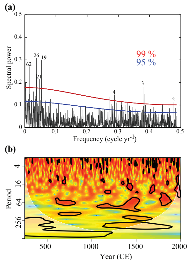
Figure 5. (a) Spectral analysis of the varve thickness series (Schulz and Mudelsee, 2002). (b) Wavelet analysis: black boundaries show the 95 % confidence level based on a red noise process. White shading represents the cone of influence where edge effects might be important.
