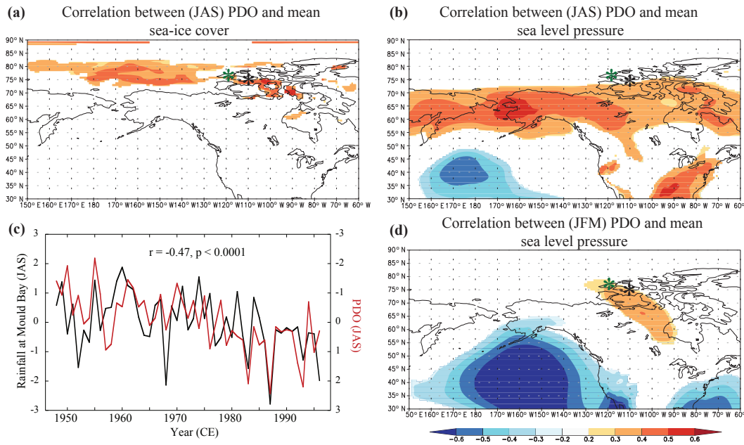
Figure 1. PDO modulation of western Canadian Arctic climate. (a) Correlation between PDO (Huang et al., 2015) and sea-ice anomalies from ERA-Interim (Dee et al., 2011) for July–September during 1979–2016. (b) Same as (a) but for mean sea level pressure from ERA-Interim (Dee et al., 2011). (c) Comparison between the time series of rainfall at Mould Bay and PDO during July–September. (d) Same as (b) but for January–March (JFM). Black and green asterisks denote Cape Bounty and Mould Bay weather stations respectively. Note that Mould Bay weather station stopped operating in 1996.
