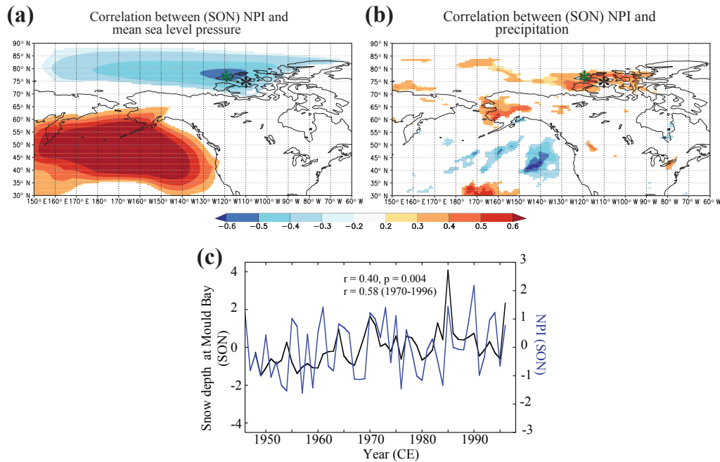
Figure 2. North Pacific Index (NPI) and precipitation during September–November. (a) Correlation between NPI (Trenberth and Hurrell, 1994) and mean sea level pressure from 1979 to 2015. (b) Same as (a), but for precipitation anomalies (Dee et al., 2011) correlated with NPI index. Black and green asterisks denote Cape Bounty and Mould Bay weather stations respectively. (c) Comparison between the time series at Mould Bay snow depth and NPI during September–November (Trenberth and Hurrell, 1994). Note that Mould Bay weather station stopped operating in 1996 CE.
