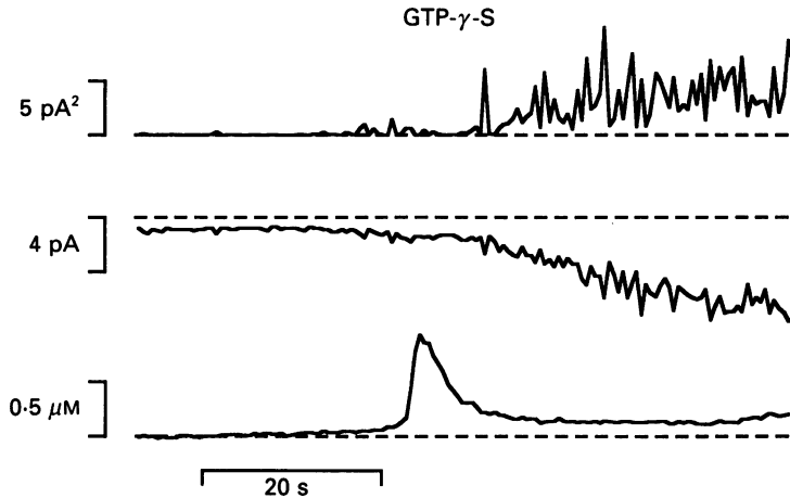
Fig. 11. Internally applied GTP- \gamma -S ( 40 \mu\text{M} ) activated the 50 pS channel and induced a \text{Ca}^{2+} transient. Top trace, variance of the membrane current. Middle trace, whole-cell membrane current. Bottom trace, [\text{Ca}^{2+}]_i .
