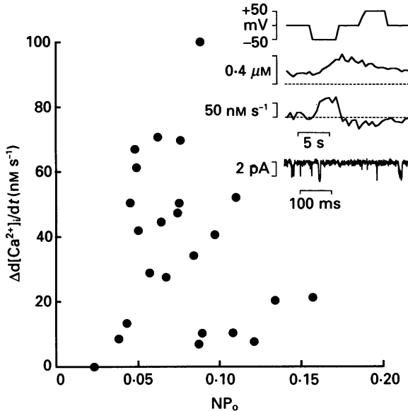
Fig. 6. Relation between \text{Ca}^{2+} influx and proportion of time that the 50 pS channel was open for an experiment with 4 \mu\text{M} internal \text{Ins}1,4,5\text{P}_3 . The protocol of voltage pulses was as in Fig. 3, with 4 s alternating positive and negative pulses, separated by 4 s periods of 0 mV. Each data point shows the result for a single negative pulse in the series. The d[\text{Ca}^{2+}]_i/dt was calculated as described in Fig. 5. \text{NP}_o is the proportion of the total period during a single pulse that one or more 50 pS channels were open (there were only a few overlapping openings of multiple channels at these low levels of single-channel activity). The inset shows one pulse cycle, with the change in [\text{Ca}^{2+}]_i , d[\text{Ca}^{2+}]_i/dt , and a sample of channel activity during the hyperpolarizing pulse.
