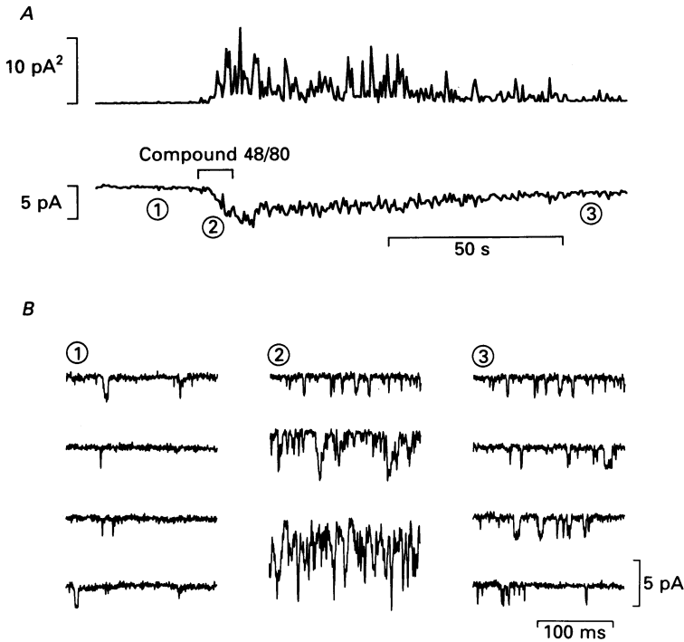
Fig. 2. Activation of large-conductance channels by compound 48/80. A , an overview of the experiment, showing the whole-cell current (bottom trace) at a steady holding potential of -50 mV. The current is smoothed by averaging over a 0.5 s sample period. The upper trace is the variance of the membrane current, calculated over the same 0.5 s periods at bandwidth 2–500 Hz. The timing of compound 48/80 application is shown above the bottom trace. B , higher resolution recordings of channel events observed in whole-cell currents. The numbers for each set of traces refer to the labelled periods in A . The traces in 1 are selected to show events; the actual rate of events was much lower during the pre-stimulation period. Bandwidth, 0–500 Hz.
