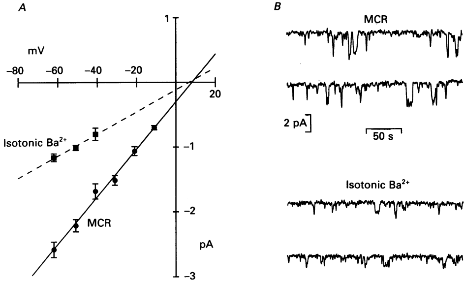
Fig. 9. A , relation between single-channel current and membrane voltage for large agonist-activated channels observed in whole-cell recordings of membrane current. Each data point is the mean of five to eleven experiments in MCR (●) or three to five experiments in isotonic \text{Ba}^{2+} (■). The vertical lines show \pm 1 standard deviation. The straight lines were fitted to the data using a least-squares criterion. Isotonic \text{Ba}^{2+} contained (in mM): \text{BaCl}_2 , 95; HEPES-NaOH, 10; glucose, 11; pH 7.2. B , examples of channel activity in MCR (upper pair of traces) and after switching the bathing solution to isotonic \text{Ba}^{2+} (lower pair of traces). Bandwidth, 0–400 Hz; membrane potential, -60 mV.
