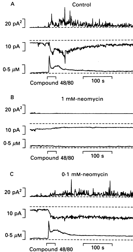
Fig. 14. Effect of internal neomycin on activation of 50 pS channels by compound 48/80. Recordings were from three mast cells in the same dish. In each group of three traces, the top is the variance of the membrane current, the middle is the membrane current, and the bottom is [\text{Ca}^{2+}]_i . A , standard intracellular solution. B , standard internal solution with 1 mM-neomycin added. C , standard internal solution with 0.1 mM-neomycin. Compound 48/80 was applied as indicated. Holding potential, -50 mV. Dashed lines indicate zero levels.
