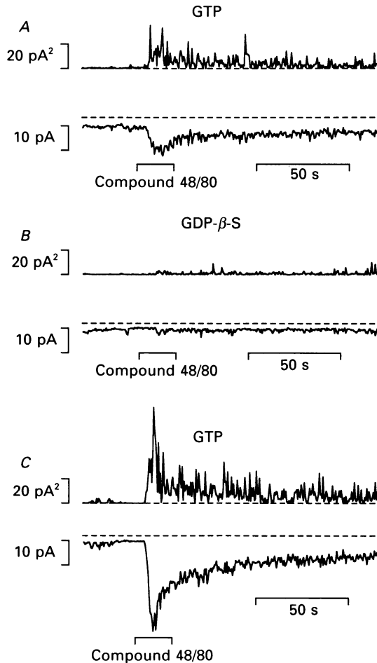
Fig. 12. Inhibition by GDP- \beta -S of the activation of 50 pS channels by compound 48/80. The pairs of traces show recordings from three consecutive cells from the same group of mast cells with 0.3 mM-GTP (A), no GTP and 0.2 mM-GDP- \beta -S (B), and 0.3 mM-GTP again (C). The bottom trace of each pair is the membrane current, and the top trace is the variance of the current, as in Fig. 2. Compound 48/80 was applied as indicated. Holding potential, -50 mV. The pipette solution contained 2 mM- \text{K}_2 -EGTA to maintain [\text{Ca}^{2+}]_i at a low level.
