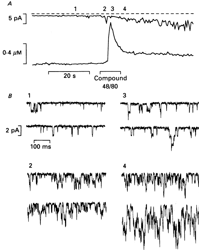
Fig. 10. Inhibition of 50 pS channel activity during Ca^{2+} transient. A , an overview of the experiment. The upper trace shows whole-cell membrane current and the lower trace [Ca^{2+}]_i in response to external application of compound 48/80 at the indicated time. B , samples of single-channel activity from the times indicated by the corresponding numbers in A . Pair 1, activity in the resting state before stimulation. Pair 2, increased activity of 50 pS channels after applying compound 48/80 but before the Ca^{2+} transient. Pair 3, inhibition of activity during the Ca^{2+} transient. Pair 4, after the Ca^{2+} transient subsided, large activation of 50 pS channels was apparent. Holding potential, -40 mV. Bandwidth, 0–400 Hz.
