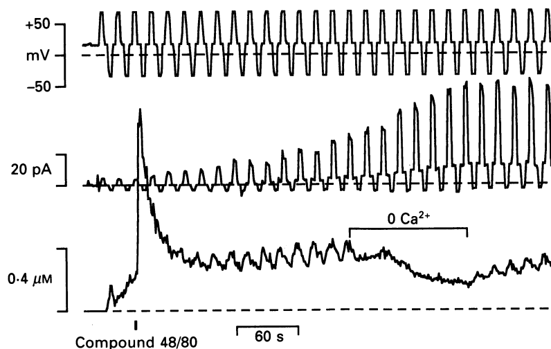
Fig. 1. Effect of compound 48/80 on membrane current and [Ca^{2+}]_i in a mast cell. The bottom trace shows [Ca^{2+}]_i as calculated from Fura-2 fluorescence, the middle trace shows the whole-cell membrane current, and the top trace shows the protocol of voltage-clamp command pulses. In each trace, the dashed line indicates the zero level. At the indicated time on the bottom trace, the mast cell secretagogue compound 48/80 ( 5 \mu M ml^{-1} ) was applied, causing a large, transient rise in [Ca^{2+}]_i . Following the transient, each negative voltage pulse was associated with an increase in [Ca^{2+}]_i . For the indicated time, the external solution was switched from MCR to a similar solution without added Ca^{2+} or Mg^{2+} .
