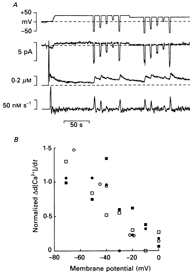
Fig. 5. Dependence of \text{Ca}^{2+} influx on membrane potential in the presence of internal \text{Ins}1,4,5\text{P}_3 . A , an example of an individual experiment. From top to bottom, the traces show the voltage protocol, the whole-cell membrane current, the calculated [\text{Ca}^{2+}]_i , and the first time-derivative of the [\text{Ca}^{2+}]_i trace ( \text{d}[\text{Ca}^{2+}]_i/\text{d}t ). Dashed lines indicate zero levels. B , summary of results of four experiments like that of A (each symbol represents a different cell). The abscissa gives the voltage during the test pulses, and the ordinate is the change in \text{d}[\text{Ca}^{2+}]_i/\text{d}t produced by each pulse ( \Delta\text{d}[\text{Ca}^{2+}]_i/\text{d}t , measured by subtracting the value of \text{d}[\text{Ca}^{2+}]_i/\text{d}t during a 1.5 s period just before each pulse from the value of \text{d}[\text{Ca}^{2+}]_i/\text{d}t in the 1.5 s period just before the end of each pulse). To compare results across experiments, the \text{d}[\text{Ca}^{2+}]_i/\text{d}t values for each cell were divided by the measured value at -60 mV.
