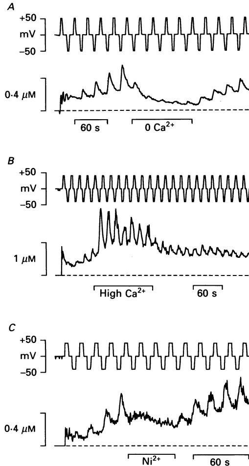
Fig. 3. \text{Ca}^{2+} influx stimulated by internal \text{Ins1,4,5P}_3 . The bottom trace of each pair is [\text{Ca}^{2+}]_i calculated from Fura-2 fluorescence, and the upper trace is the voltage protocol. The dashed baseline indicates the zero level. A , 0.5 \mu\text{M-Ins1,4,5P}_3 . At the time indicated, the bath solution was changed from MCR to the same solution without added \text{Ca}^{2+} or \text{Mg}^{2+} . B , 10 \mu\text{M-Ins1,4,5P}_3 . The external solution was switched from MCR to Ringer solution with 5 \text{ mM-Ca}^{2+} and 0.5 \text{ mM-Mg}^{2+} at the indicated time. C , 10 \mu\text{M-Ins1,4,5P}_3 . The external solution was changed from MCR to \text{MCR} + 5 \text{ mM-Ni}^{2+} at the indicated time.
