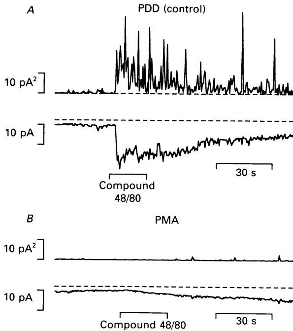
Fig. 13. Effect of phorbol esters on activation of 50 pS channels by compound 48/80. Recordings were from two mast cells in the same preparation. A , incubation for 31 min in MCR containing 0.1 \mu M-PDD (an inactive phorbol ester). Upper trace shows the variance of the membrane current, as in Fig. 2, and the lower trace is the membrane current. Timing of compound 48/80 application was as indicated. Holding potential, -50 mV. Internal solution contained 2 mM-K 2 -EGTA. B , as in A , except that the cell was incubated for 32 min in MCR containing 0.1 \mu M-PMA.
