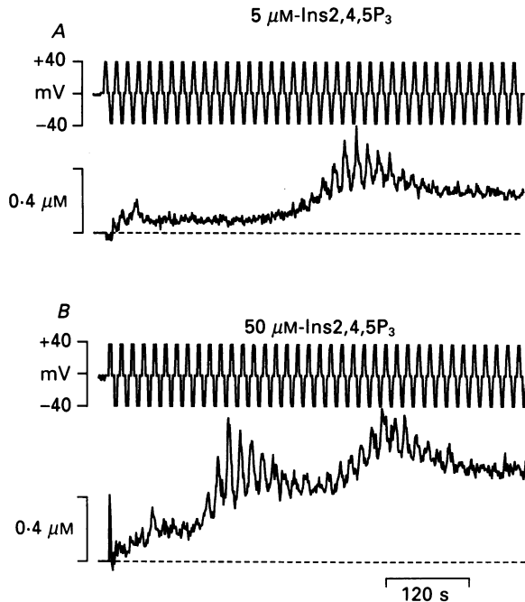
Fig. 4. Ca^{2+} influx stimulated by internal Ins2,4,5P_3 . The bottom trace of each pair is [Ca^{2+}]_i calculated from Fura-2 fluorescence, and the upper trace is the voltage protocol. The dashed baseline indicates the zero level. A, 5 \mu M-Ins2,4,5P_3 . B, 50 \mu M-Ins2,4,5P_3 .
