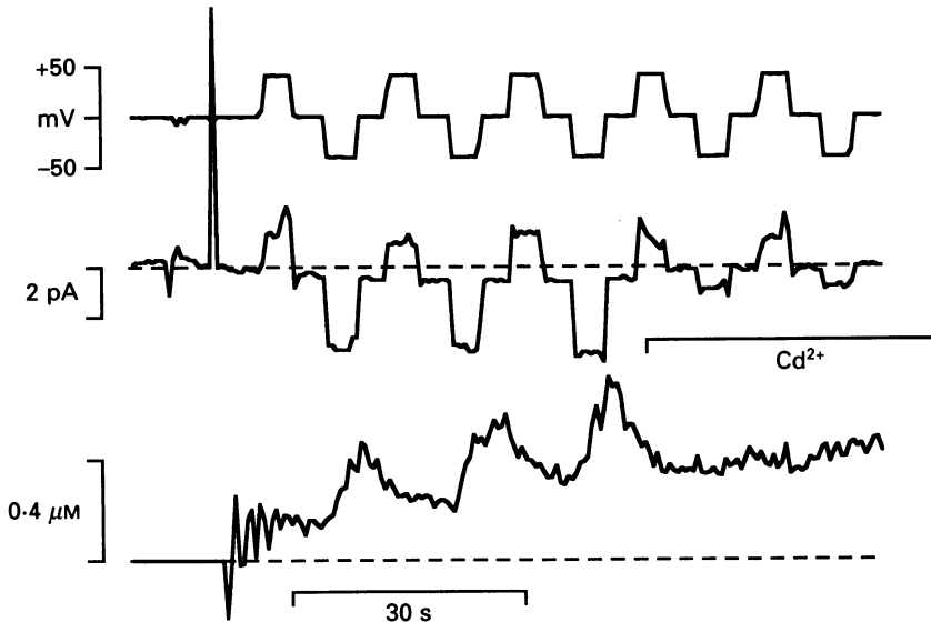
Fig. 8. Effect of cadmium on membrane current and \text{Ca}^{2+} influx induced by \text{Ins}1,4,5\text{P}_3 . Top trace: voltage protocol; middle trace: whole-cell membrane current; bottom trace: [\text{Ca}^{2+}]_i . Dashed lines indicate zero levels. Internal solution contained 10 \mu\text{M} - \text{Ins}1,4,5\text{P}_3 , and the external solution was MCR. Both internal and external solutions contained 10 \mu\text{M} -DIDS to block \text{Cl}^- current. The time of breaking into the cell is marked by the large artifact near the beginning of the current trace. At the indicated point, the bath was perfused with MCR containing 5 \text{ mM} - \text{Cd}^{2+} .
