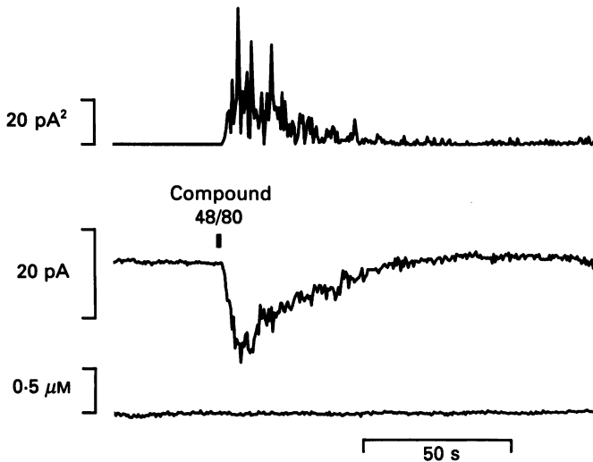
Fig. 7. Lack of effect of internal \text{Ins}1,4,5\text{P}_3 , \text{Ins}1,3,4,5\text{P}_4 and EGTA on activation of the 50 pS channel by compound 48/80. The pipette solution contained 10\ \mu\text{M} - \text{Ins}1,4,5\text{P}_3 , 10\ \mu\text{M} - \text{Ins}1,3,4,5\text{P}_4 and 2\ \text{mM} - \text{K}_2 -EGTA to clamp [\text{Ca}^{2+}]_i near zero (bottom trace). Application of compound 48/80 at the indicated time activated a large whole-cell membrane current (middle trace), consisting of superimposed activity of many 50 pS channels. The upper trace is the variance of the membrane current, calculated as in Fig. 2. The steady holding potential was -50\ \text{mV} .
