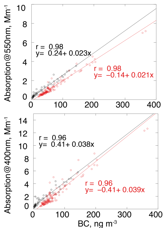
Figure 13. Scatterplot of observed (black) and simulated (red) absorption at 550 nm (top) and 400 nm (bottom) vs. BC concentrations from at ATTO in January–April 2014. Correlation coefficients and slopes of reduced-major-axis (RMA) regressions are shown as inset.
