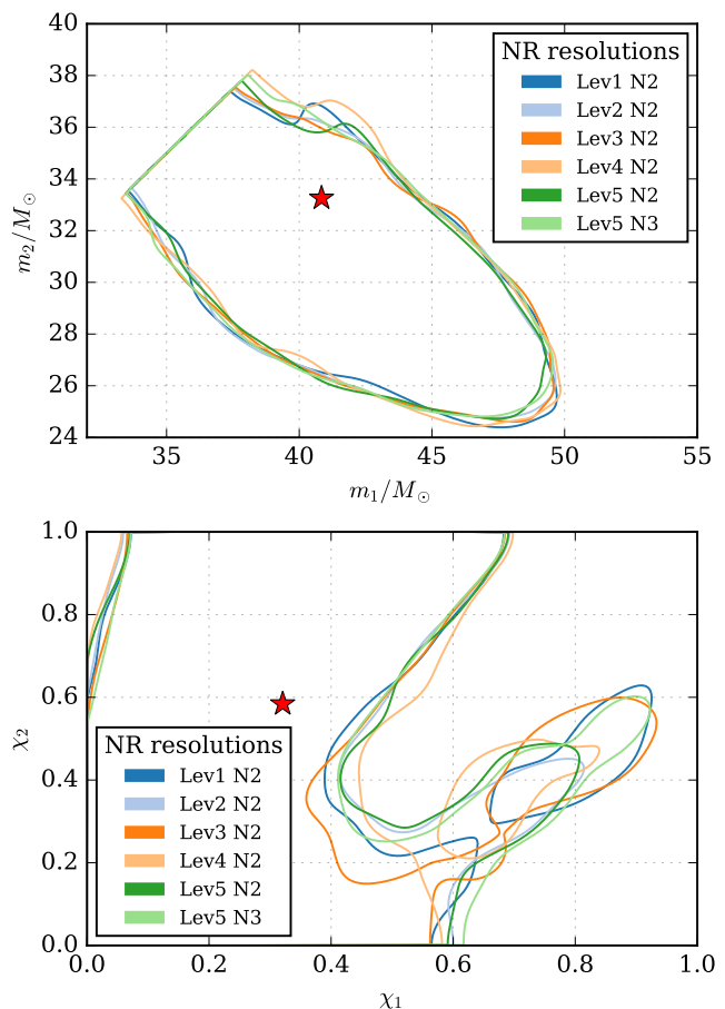
FIG. 9. 90% credible regions for configuration SXS:BBH:0308 with numerical resolutions \text{Lev} = \{1, 2, 3, 4, 5\} and extrapolation orders N = \{2, 3\} . We find consistent results between the different resolutions and extrapolation orders, indicating that numerical errors are a negligible source of parameter biases.
