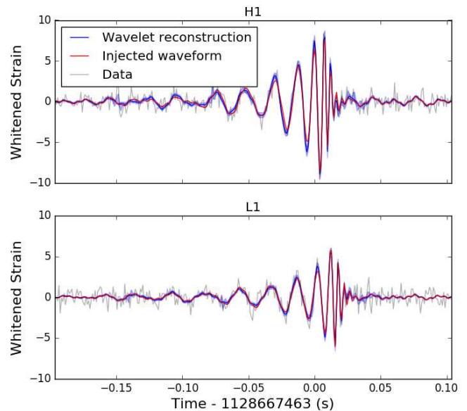
FIG. 8: BayesWave median reconstruction and 90% credible interval (blue) and the injected waveform (red), time is shown on the x -axis and whitened strain on the y -axis. The data has been whitened using the estimated noise curve from the time of the injection. The network match for this waveform is 98%.
