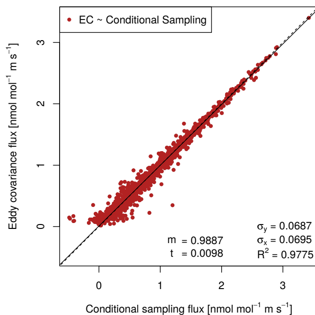
Figure 1. Scatterplot of conditional sampling against eddy covariance methane flux for times with best steady state conditions and well developed turbulence. The dashed line follows the function f(x) = x and the solid one is the orthogonal regression line.
