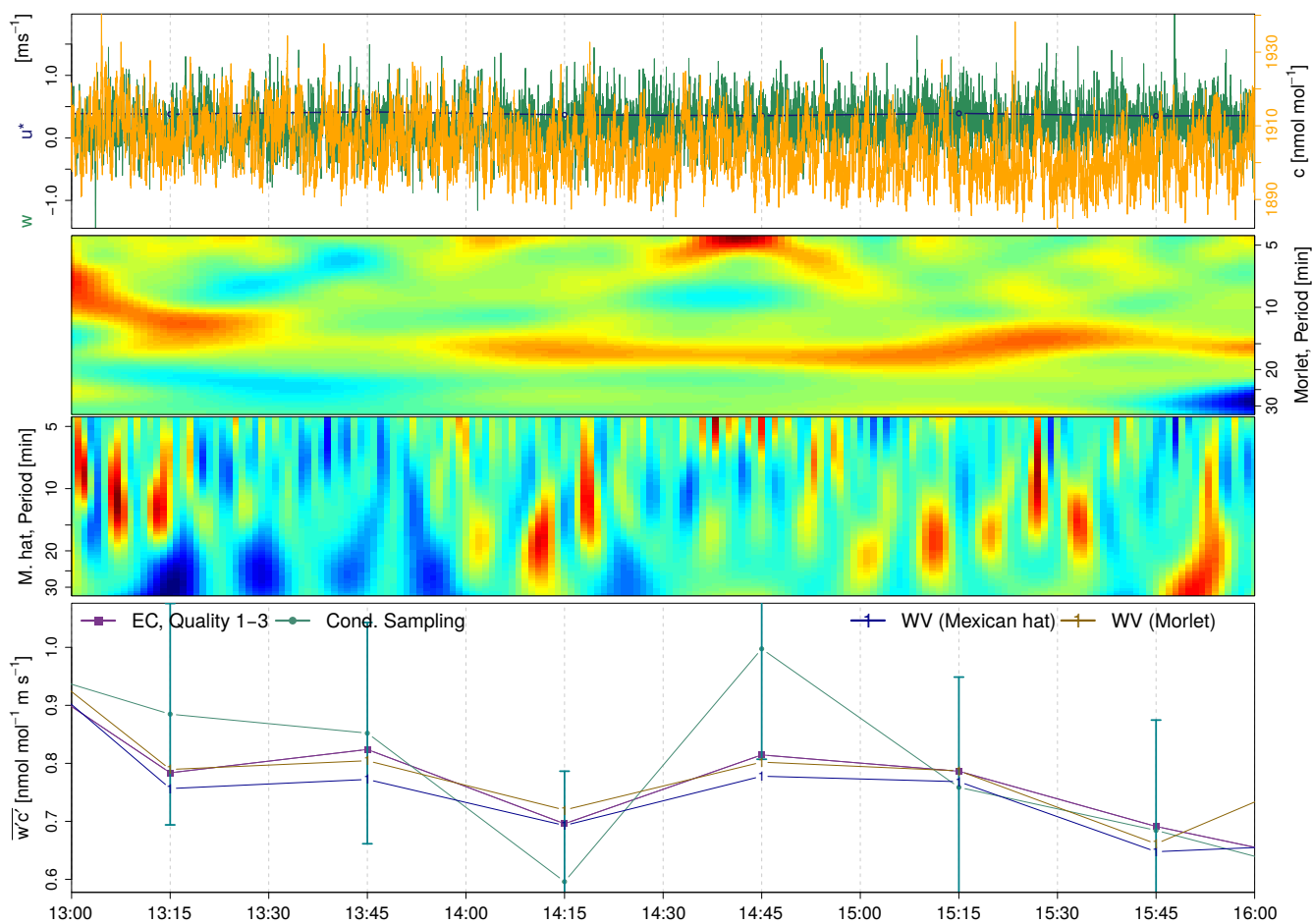
Figure 4. Case study of 23.07.2014. The colours in the wavelet cross-scalograms between w and c denote the flux intensity, blue refer to the smallest, green to medium and red to highest methane flux contributions. The cone of influence is outside of the scalogram, i.e., it was not affected by border effects. The error bars for conditional sampling display the range of the result for \bar{w} \pm 10^{-4} \text{ ms}^{-1} .
