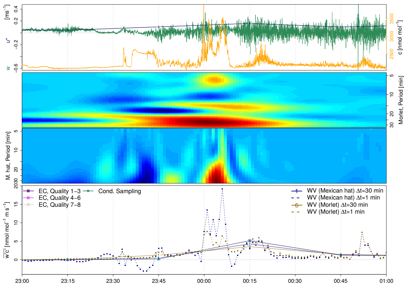
Figure 5. Case study of 02./03.08.2014. The colours in the wavelet cross-scalograms between w and c denote the flux intensity, blue refer to the smallest, green to medium and red to highest methane flux contributions. The cone of influence is outside of the scalogram, i.e., it was not affected by border effects. Dashed lines represent wavelet fluxes with an averaging period of 1 min. The error bars for conditional sampling display the range of the result for \bar{w} \pm 10^{-4} \text{ ms}^{-1} .
