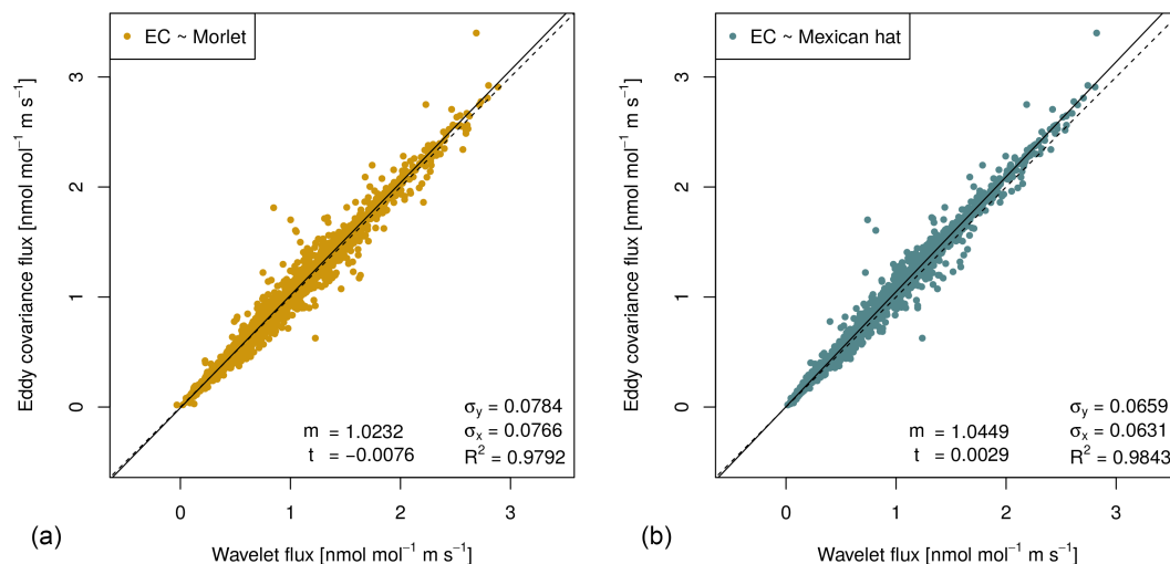
Figure 3. Scatterplot of Morlet (left) and Mexican hat wavelet methane flux (right) against eddy covariance for times with best steady-state conditions and well-developed turbulence. The dashed line follows the function f(x) = x and the solid one is the mean regression line.
