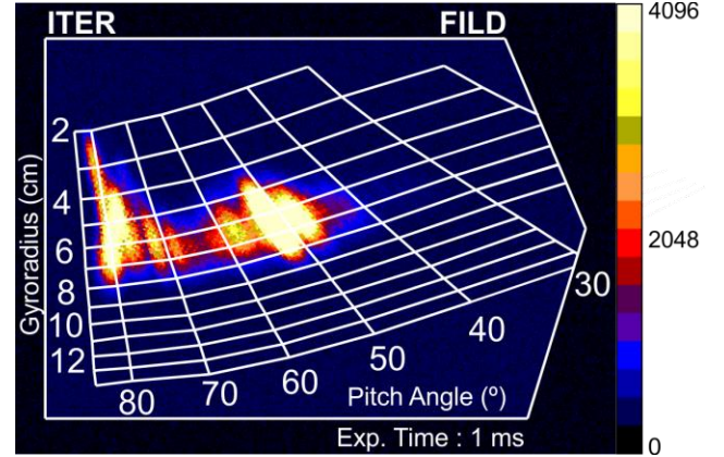
Figure 5. Synthetic measurement of alpha particle losses induced by RMPs with the present design of the ITER FILD.
