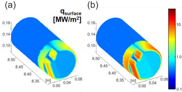
Figure 4. Expected heat load on the FILD detector head in the ITER 15 MA scenario calculated with the field line tracing code PFCFLUX for two different separatrix positions at \Delta_{\text{FILD-port}} = 11\text{cm} ; (a) nominal separatrix and (b) 5.5 cm outwards shift of the separatrix to account for the worst-case magnetic perturbation of the plasma boundary and magnetic reconstruction error.
