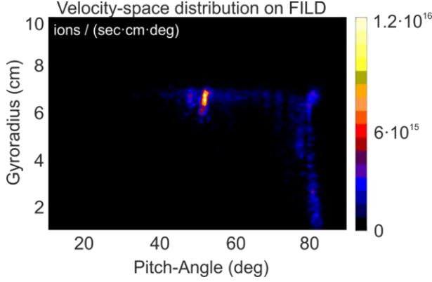
Figure 2. ASCOT Simulations. Velocity-space of alpha particle losses hitting the FILD detector head in the presence of an externally applied n = 4 RMP.
