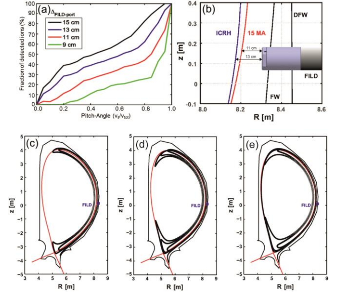
Figure 3. ASCOT Simulations. Backwards full orbit simulations. (a) Pitch-Angle coverage at different detector head radial positions. (b) Optimal detector head position with respect to separatrix for the standard and ICRH optimized 15 MA scenario. (c)-(e) Test orbits of 3.5 MeV alpha particles followed backwards in time for 3 different positions of detector head; \Delta_{\text{FILD-port}} = 11, 13 and 14 cm respectively.
