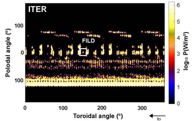
Figure 1. ASCOT simulations of alpha particle heat load in ITER on a 3D first wall due to an externally applied n=4 RMP. The location of the FILD head is indicated with a white box.
