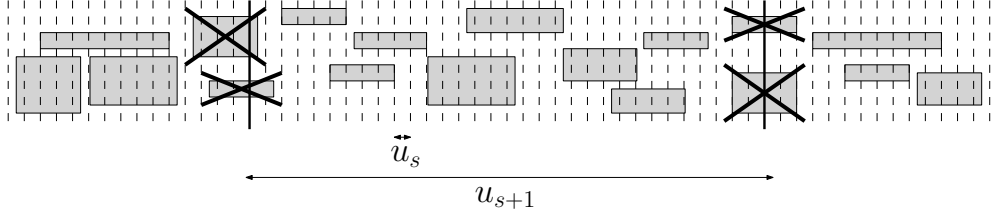
Figure 1: The vertical grid. The dashed vertical lines are the vertical grid lines of G_s^V , the bold vertical lines are the lines in the set G_{s+1}^V . All shown rectangles are from level \mathcal{R}_s^V . The crossed out rectangles are abusive since they intersect lines from G_{s+1}^V .
