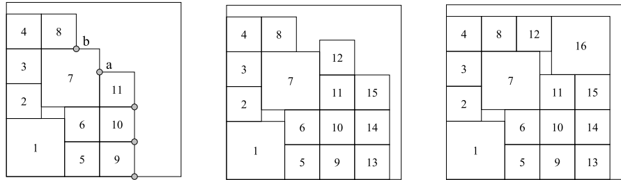
(a) Situation after packing the first 11 items (b) Continuing with the next available position (c) Leaving out the next available position
