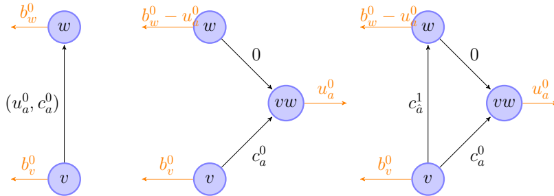
Figure 1: The transition from the left to the middle, which is done for each arc, removes the capacity constraint. From the middle to the right: In order to balance the x_a s_a , we introduce the arc \hat{a} = (v, w) with high cost c_{\hat{a}} and reroute flow along it. The direction of \hat{a} depends on a tree solution z in the original graph. It is flipped if z_a \leq u_a/2 . All arcs in the middle and the right graph have infinite capacity. Only the costs are shown.
