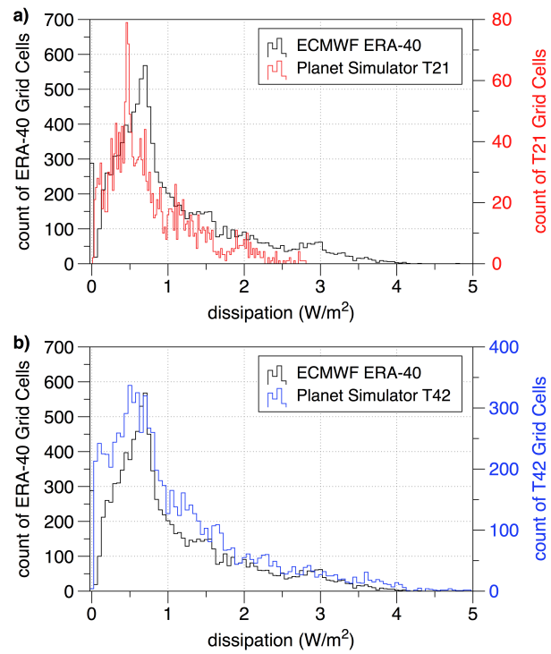
Figure 2.4: Global mean dissipation values for a) ERA-40 and a T21 10-vertical layer simulation and b) ERA-40 and T42 10-vertical layer simulation.
