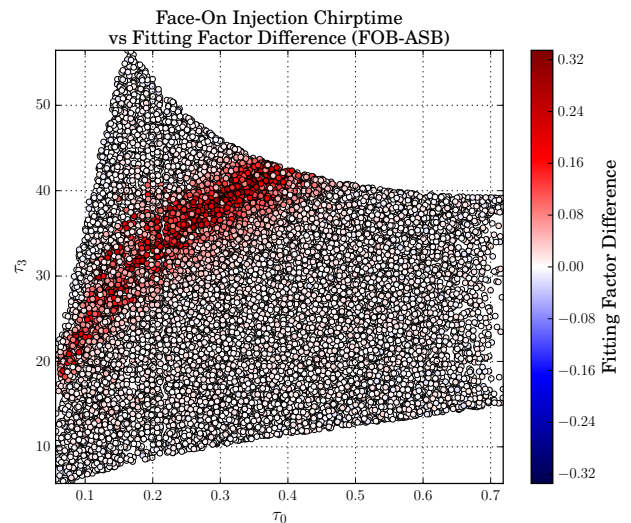
FIG. 12. A plot of the difference in the recovered fitting factor between the precessing and aligned template banks over the \{\tau_0, \tau_3\} parameter space for face-on SpinTaylorF2 injections.
