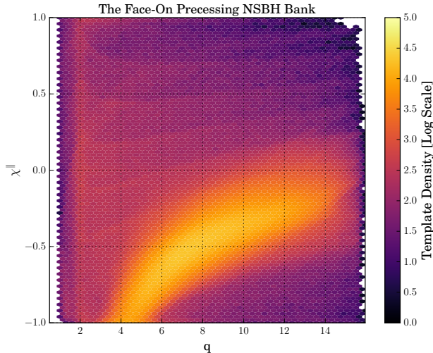
FIG. 5. The FOB in (q, \chi^{\parallel}) coordinates. As before, the color bar is scaled with respect to the density of templates per hexbin \{\Delta q = 0.3, \Delta \chi^{\parallel} = 0.04\} .
