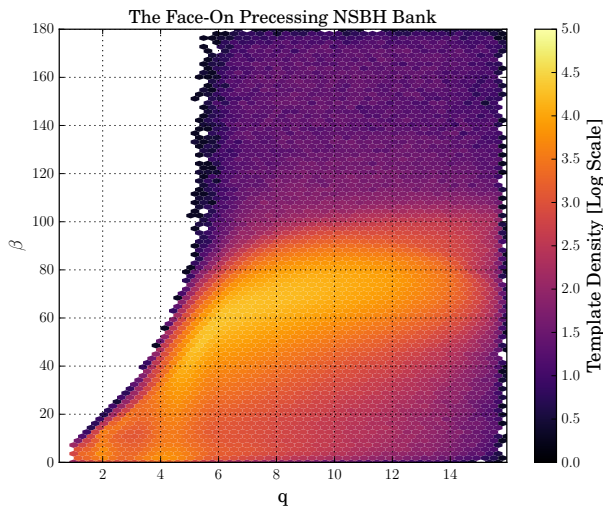
FIG. 7. The \beta and mass ratio, q , distribution of the FOB. Each hexbin has dimensions \{\Delta q = 0.3, \Delta \beta = 4^\circ\} .
