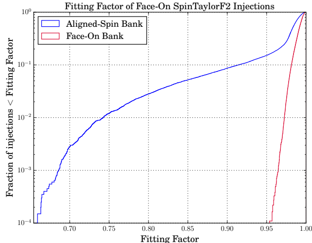
FIG. 10. Cumulative histogram showing the recovered fitting factor of the face-on-precessing and aligned spin template banks for face-on SpinTaylorF2 injections.
