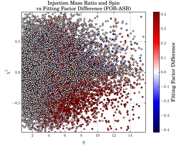
FIG. 15. A plot of the difference in the recovered fitting factor between the precessing and aligned template banks over the \{q, \chi^\parallel\} parameter space for SpinTaylorF2 injections with arbitrary orientations of \mathbf{J} .
