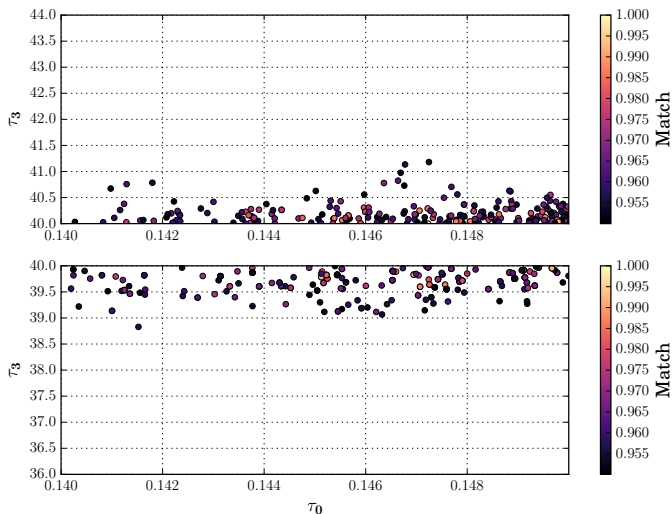
FIG. 8. Plot of the templates in the box (\tau_0, \tau_3) = (0.14 - 0.15, 40 - 44) that had an overlap greater than 95% with templates placed in the box, (\tau_0, \tau_3) = (0.14 - 0.15, 36 - 40) .
