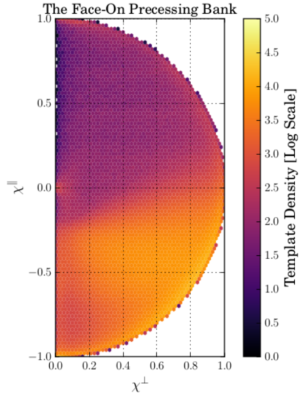
FIG. 6. The spin distribution of the FOB. The y-axis is the component of spin parallel to the orbital angular momentum \mathbf{L} and the x-axis is the component of the spin perpendicular to \mathbf{L} . Each hexbin has dimensions \{\Delta \chi^{\parallel} = 0.04, \Delta \chi^{\perp} = 0.02\} .
