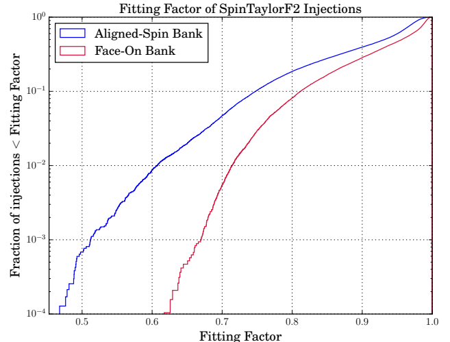
FIG. 11. Cumulative histogram showing the recovered fitting factor of the face-on-precessing and aligned spin template banks for SpinTaylorF2 injections with arbitrary values of \theta_J .
