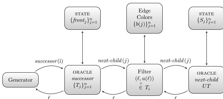
■ Figure 2 Generator for next-neighbor queries in BA_n (the generator is input a query for a next-neighbor of vertex i from the right)
