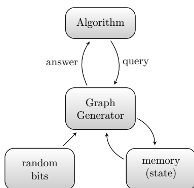
■ Figure 1 A random access graph generator
