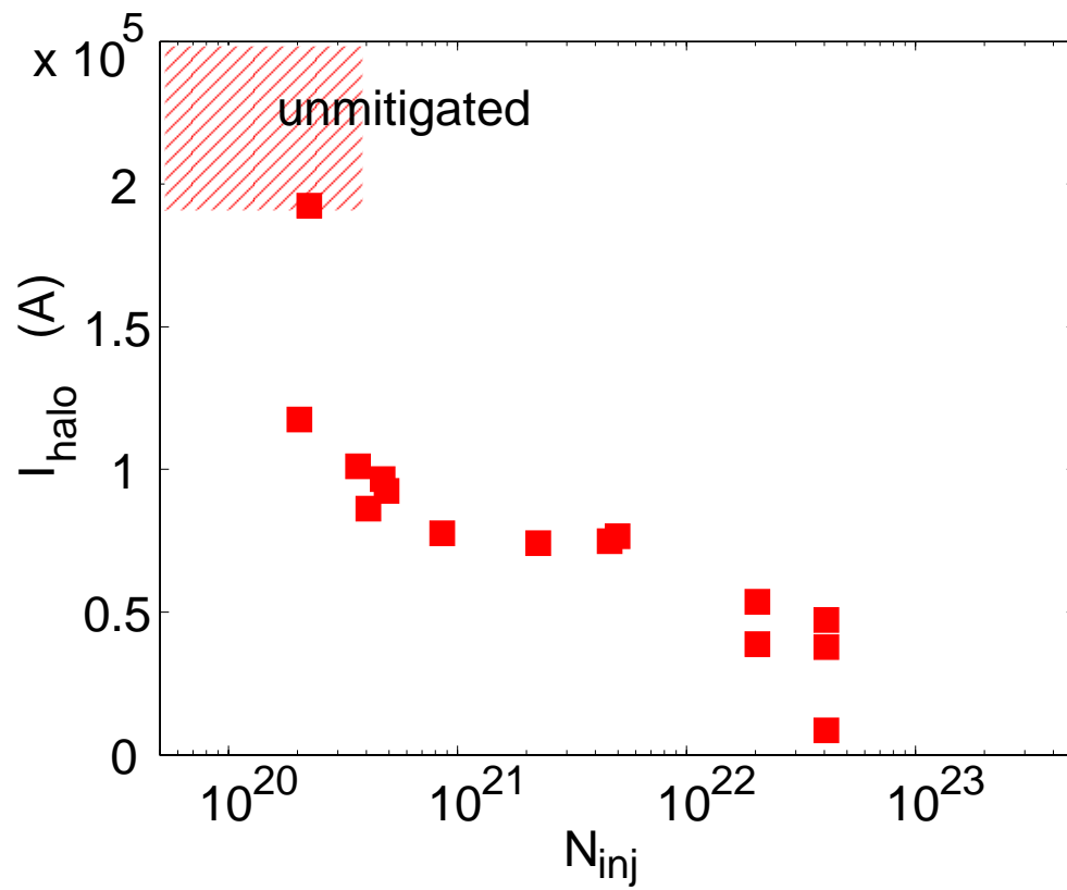
Figure 5: Halo current ( I_{halo} ) versus the number of injected neon atoms ( N_{inj} ).
