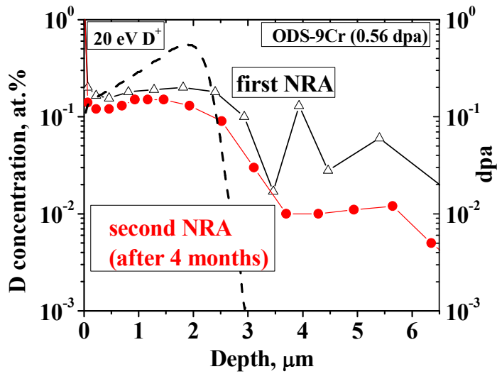
Fig. 8. Depth profiles of D in ODS-9Cr steel pre-damaged with 20 MeV W ions up to 0.56 dpa and subsequently exposed to the D plasma with incident ion energy of 20 eV per D at room temperature up to a fluence of 2.9 \times 10^{25} D/m 2 . The measurements were performed in two weeks and four months after the D plasma exposure.
