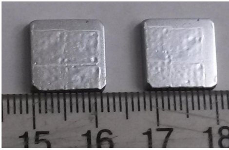
Fig. 1. Samples after damaging with e-beam in JUDITH-1. Pulse duration is \Delta t=1 ms, absorbed power density is 0.71 \text{ GW/m}^2 , and pulse number is 10.
