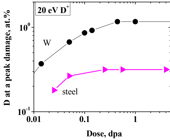
Fig. 9. The D concentration at a peak damage in steel and tungsten samples pre-irradiated with 20 MeV W ions at room temperature as a function of dpa.
