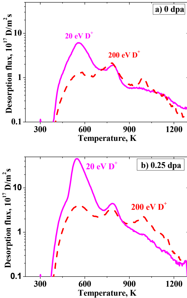
Fig. 11. Thermal desorption spectra of D from Eurofer samples after exposure to the D plasma with incident ion energy of 20 and 200 eV per D at room temperature up to a fluence of 6 \times 10^{24} \text{ D/m}^2 . (a) undamaged Eurofer and (b) Eurofer pre-damaged with 20 MeV W ions up to 0.25 dpa.
