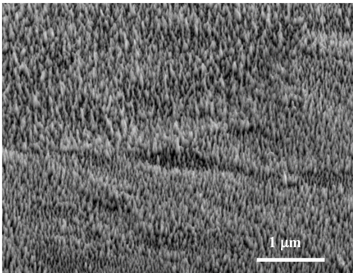
b) Undamaged Eurofer (0 dpa), RT
