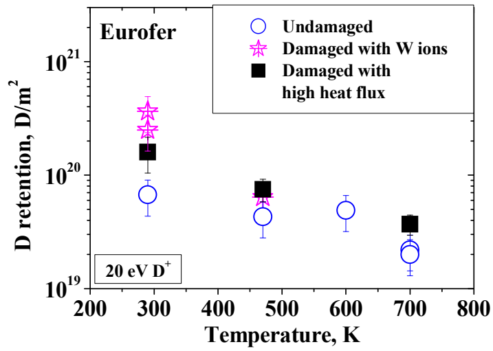
Fig. 15. A comparison of the D retention in undamaged Eurofer with Eurofer pre-damaged with W ions and high heat flux and sequentially exposed to the D plasma with 20 eV per D up to a fluence of 6 \times 10^{24} D/m 2 .
