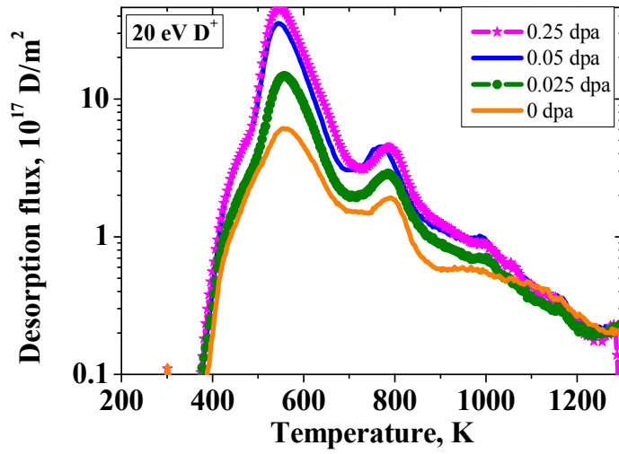
Fig. 12. Thermal desorption spectra of D from Eurofer samples pre-damaged with 20 MeV W ions at different dpa and subsequently irradiated with 20 eV per D at room temperature up to a fluence of 6 \times 10^{24} D/m 2 .
