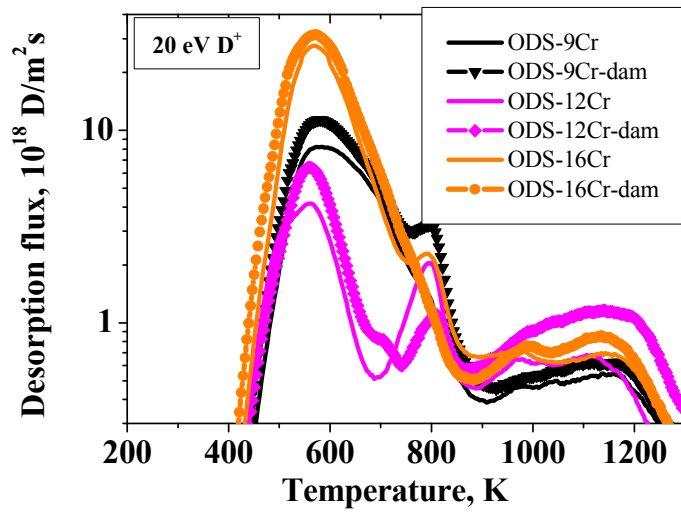
Fig. 13. Comparison of thermal desorption spectra of D in undamaged ODS steels and pre-damaged with 20 MeV W ions up to 0.56 dpa (marked as ODS-dam) and subsequently irradiated with 20 eV per D at room temperature up to a fluence of 2.9 \times 10^{25} D/m 2 .
