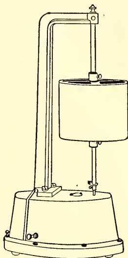
FIG. 30. Clockwork Kymograph.
