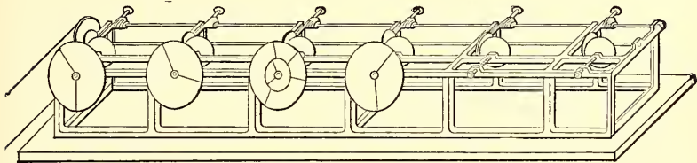
FIG. 4. Demonstrational Colour Mixer, for six sets of discs.
