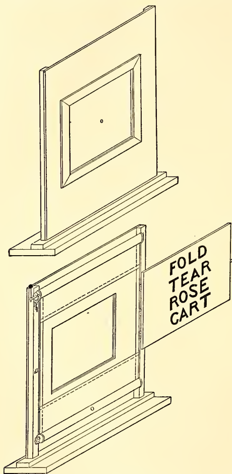
FIG. 42. Demonstrational Tachistoscope. A black curtain, mounted on strong spring rollers, is stretched behind a square opening in a black wooden screen. The upper Fig. (front) shows the curtain and the white fixation-mark. The lower Fig. (back) has the card-carrier thrown back to show the square opening in the curtain itself.
