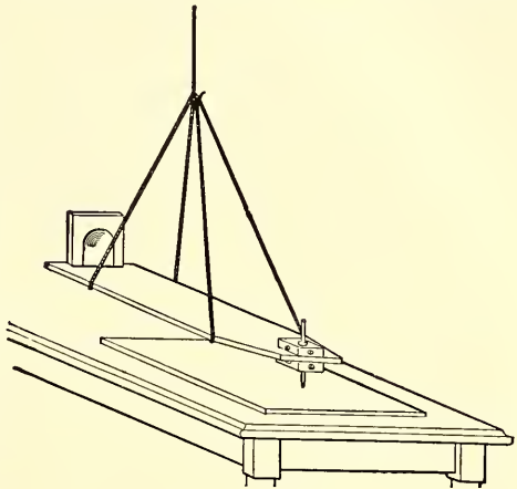
FIG. 34. Automatograph.
