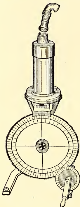
FIG. 15. Stern's Variator.
