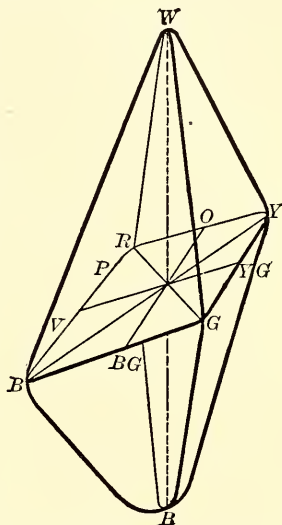
FIG. 2. The Colour Pyramid.
