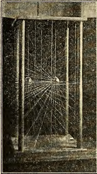
FIG. 45. Horopter Model, showing the horopter as a horizontal circle and a vertical through the fixation-point.
