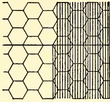
FIG. 54. A field of cones (shown schematically as hexagons) is stimulated by a sheet of half-white and half-black paper.
