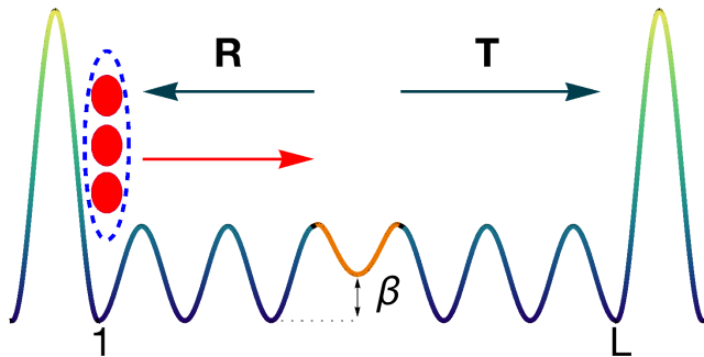
FIG. 1. Scheme of the model: when a bound state is initially in the site 1 of a finite lattice, a suitably introduced local impurity (orange) in the chemical potential \mu_j = -\beta\delta_{j,L/2+1} triggers a wave-packet splitting in a reflected R and a transmitted T component. If appropriately tuned it generates a NOON state between the endpoints (site 1 and L ) at the transfer time. The two green peaks are local fields which realize a finite lattice model. The red arrow represents the natural direction of propagation of the bound particle once lowered the lattice depth at time t = 0 . We also add local fields in the first and last sites of the chain to inhibit the edge-localization effect and then to delocalize the bound particle from the edges.
