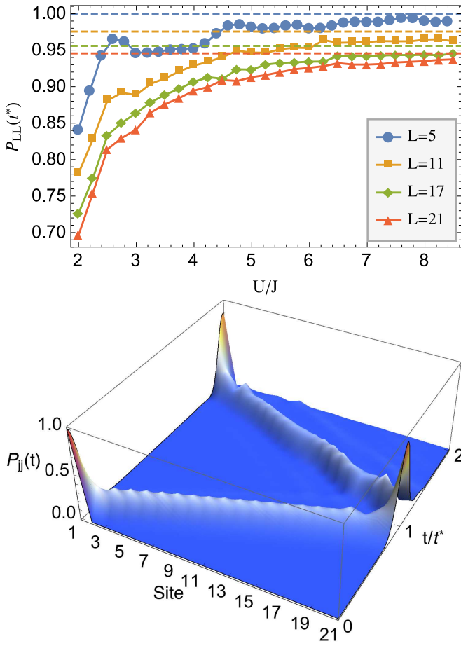
FIG. 3. Optimal transfer of a two particle bound state: (top) analysis of the transfer fidelity P_{LL}(t^*) for the initial state |\psi(0)\rangle \propto (a_1^\dagger)^2|0\rangle as a function of the onsite interaction U/J when the optimal transfer scheme J_1 = J_L = J_0 and J_j = J for j \neq (1, L) is included in the model 1. Here we also add two local impurities \mu_j = -\beta_1(\delta_{j,1} + \delta_{j,L}) and \mu_j = -\beta_2(\delta_{j,2} + \delta_{j,L-1}) where \beta_1 = (J_0^2 - 2J^2)/2U and \beta_2 = (J_0^2 - J^2)/2U to eliminate the edge-locking effect. The J_0 value is chosen by numerically maximizing the transfer fidelity in a single particle manifold [61]. To compare the difference between a single particle and a bound state, we plot (with a dashed line) also the single-particle transfer fidelity P_L(t^*) = |\langle 0|a_L|\psi(t^*)\rangle|^2 obtained for a system initially in a_1^\dagger|0\rangle . (bottom) Probability P_{ij}(t) to have a two particle bound state in site j at time t/t^* for a minimal engineered chain with L = 21 and U/J = 8 .
