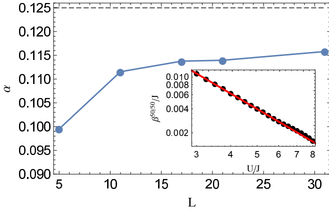
FIG. 9. Finite-size effects in the three particle NOON state generation: analysis of the scaling factor \alpha as a function of the chain length L for a three particle bound state, where \beta^{50/50} = \alpha J^3 / U^2 . The dashed grey line represents the theoretical value from the effective Hamiltonian description. (Inset) Analysis of the optimal value of \beta to produce the NOON state with three particles as a function of U/J in a uniform chain with length L = 5 . The red line is the fit \beta^{50/50} = \alpha J^3 / U^2 where \alpha = 0.099 .
