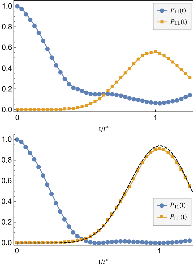
FIG. 2. Edge delocalization for a two particle bound state: plot of the probability to have a bound particle in the first P_{11}(t) and in the last P_{LL}(t) site as a function of the time t , scaled for the transfer time t^* \sim L/J_{\text{eff}} for a uniform chain with L = 5 and U/J = 5 in the initial state |\psi(0)\rangle \propto (a_1^\dagger)^2|0\rangle . We add a local field \mu_j = -\beta'(\delta_{j,1} + \delta_{j,L}) with strength \beta' = 0 (top), and \beta' = \beta'_{\text{opt}} = J^2/4U (bottom). To compare the results with the single particle case we plot, with a dashed black line, the probability P_L(t) = |\langle 0|a_L|\psi(t)\rangle|^2 for a single particle initially in a_1^\dagger|0\rangle (here t^* \sim L/J ).
