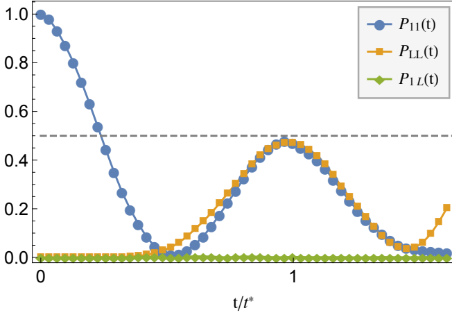
FIG. 5. Two particle NOON state: plot of the probabilities P_{ij}(t) to have one particle in site i and the other in j , as a function of the time, in unit of the transfer time t^* , for two particles initially in |\psi(0)\rangle \propto (a_1^\dagger)^2 |0\rangle . Here we consider a uniform chain with an impurity \mu_j = -\beta\delta_{j,L/2+1} where \beta = 0.789(J^2/2U) in a chain with U/J = 5 and length L = 5 . The absence of the P_{1L}(t^*) term is an evidence that the output state at t = t^* \simeq UL/J^2 is the NOON state with two particles. The grey dashed line represents the results for an ideal lossless NOON state generation.
