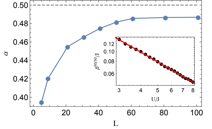
FIG. 6. Finite-size effects in the two particle NOON state generation: analysis of the scaling factor \alpha where \beta^{50/50} = \alpha J^2/U , as a function of the chain length L for generating a two particle NOON state. The grey line represents the theoretical results from the effective Hamiltonian theory, which holds for L \gg 1 . (Inset) Analysis of the optimal value of \beta of the local field \mu_j = -\beta\delta_{j,L/2+1} which produces the NOON state with two particles as a function of U/J for L = 5 . The red line is the fit \beta = \beta^{50/50} = 0.395J^2/U .
