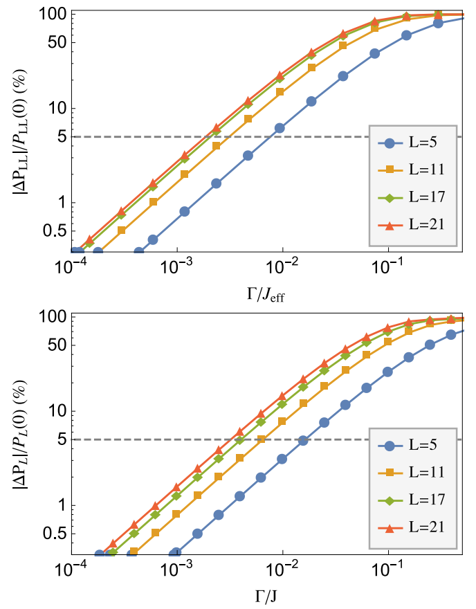
FIG. 4. Decoherence effects for a two particle bound state: (top) relative variation \Delta P_{LL}/P_{LL}(t^*, \Gamma = 0) of the transfer fidelity P_{LL}(t^*) with respect to the case in absence of decoherence, for a uniform chain with U/J = 3 and length L . Here \Delta P_{LL} = |P_{LL}(t^*, \Gamma) - P_{LL}(t^*, \Gamma = 0)| and the dashed grey line is a threshold of a relative variation of the 5%. Several chain length L are considered. (bottom) Relative variation \Delta P_L/P_L(t^*, \Gamma = 0) for a single particle state initially in a_1^\dagger|0\rangle .
