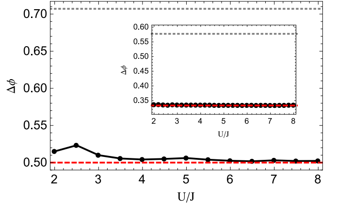
FIG. 12. Phase estimation precision \Delta\phi = 1/\sqrt{F_Q} , where F_Q is the Quantum Fisher Information for the estimator n_L in a uniform chain with L = 5 respectively for a two particle bound state and for a three particle bound state (inset), as a function of the onsite interaction U/J . The red dashed/grey dotted lines represent the ideal quantum/classical lower bound, respectively \Delta\phi_{\text{quant}} = 1/M and \Delta\phi_{\text{cl}} = 1/\sqrt{M} .
