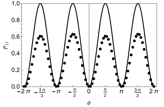
FIG. 10. NOON state detection with bound particles: interference fringes in a Mach-Zehnder scheme for a two particle bound state for a chain with L = 5 and U/J = 5 . We plot the probability P_{11}(t^*) to have the bound state particle in the first site after an time evolution for t^* \simeq LU/J^2 , when a phase factor \phi is introduced in the system. The line data represent the result for an ideal lossless Mach-Zehnder transformation.
