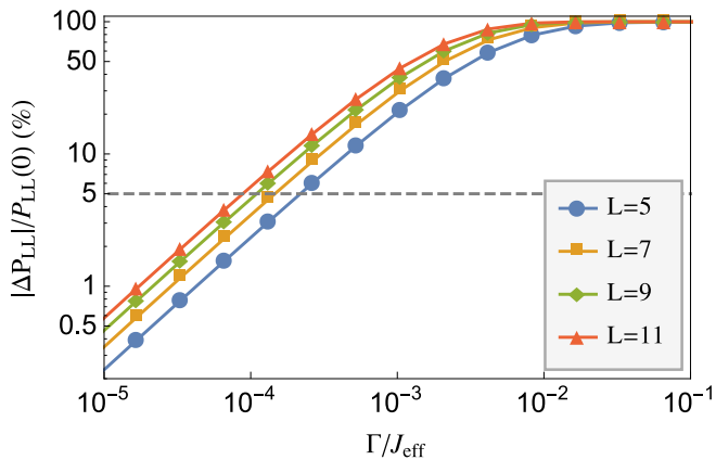
FIG. 7. Decoherence effects for a three particle bound state: relative variation \Delta P_{LL}/P_{LL}(t^*, \Gamma = 0) , with respect to decoherence free case, for a uniform chain with U/J = 2 . Here \Delta P_{LL} = |P_{LL}(t^*, \Gamma) - P_{LL}(t^*, \Gamma = 0)| and the dashed grey line is a threshold of a relative variation of the 5%. Several chain length L are considered.
