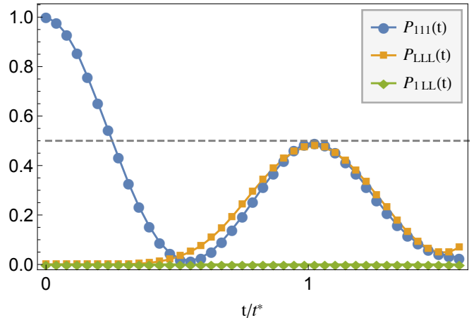
FIG. 8. Three particle NOON state: joint probabilities P_{ijk}(t) as a function of the time, in unit of the transfer time t^* , for three particles initially in |\psi(0)\rangle \propto (a_1^\dagger)^3|0\rangle for a uniform chain with an impurity \beta = 0.099J^3/U^2 and \beta' = J^2/8U in the middle of the chain with U/J = 5 and length L = 5 . The absence of the P_{1LL}(t) term is an evidence that the output state at t = t^* is the NOON state with two particles. The grey dashed line represents the results for an ideal lossless NOON state generation. We found also that P_{1LL}(t) = P_{11L}(t) .
