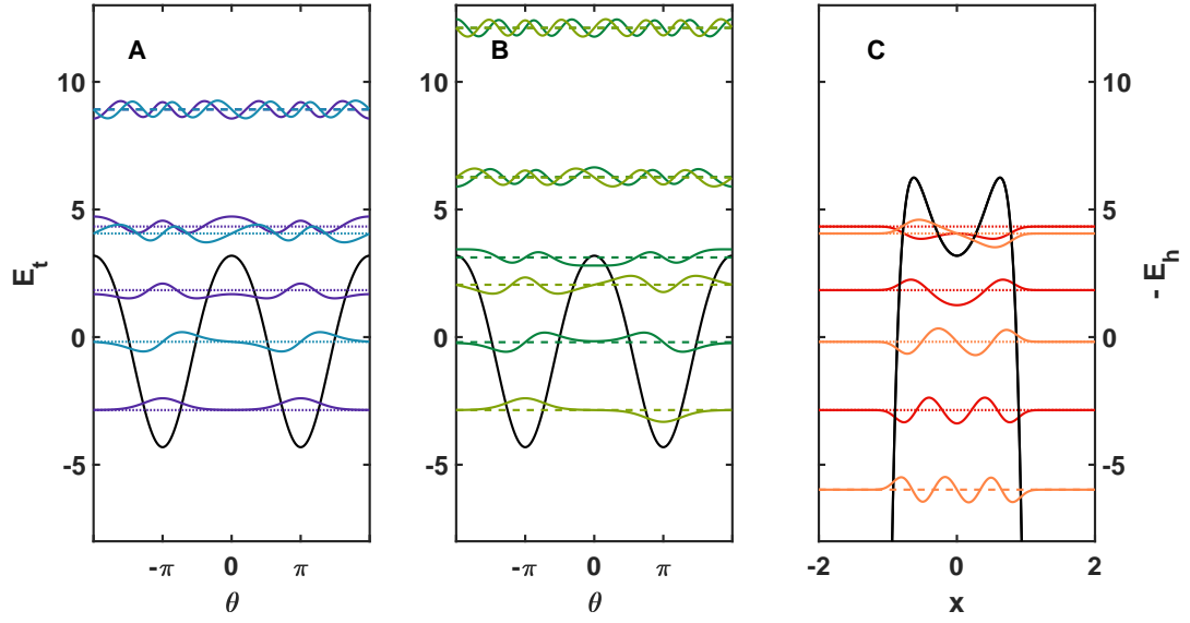
FIG. 6. Same as Fig. 4 but for \beta = -3/4 . For \kappa = 5 , the energies E_t for periodic states (A) are anti-isospectral to E_h .
