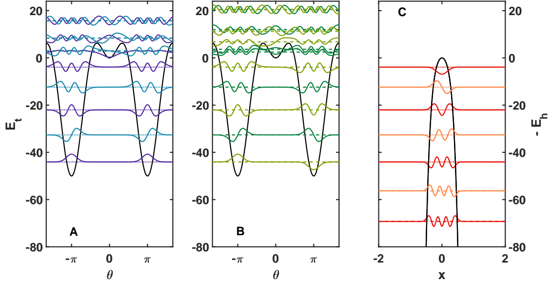
FIG. 4. Trigonometric V_t (panels A and B) and inverted hyperbolic -V_h (panel C) potentials for \beta = -5 , with analytical (dotted lines) and numerical (dashed lines) eigenenergies and wavefunctions (full curves). For \kappa = 5 , the energies E_t for periodic states (A) are anti-isospectral with Razavy energies E_h .
