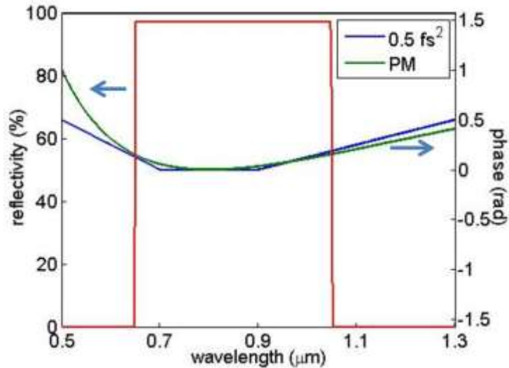
Fig. 4.32. A cavity reflection window (red) with a high reflection from 0.65 \mu\text{m} – 1.05 \mu\text{m} , the gain bandwidth of Ti:sapphire crystals; the round-trip phase profiles with 0.5 \text{fs}^2 of GDD (blue) or linear phase-matching ramps (green) below 0.7 \mu\text{m} and above 0.9 \mu\text{m} .
