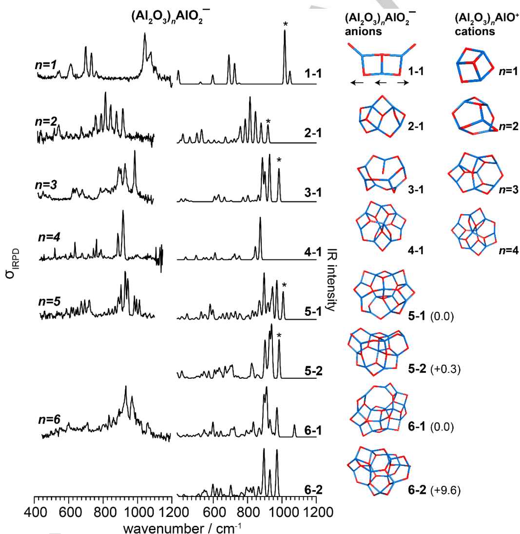
Figure 2. Experimental IRPD spectra (1 st column) of (\text{Al}_2\text{O}_3)_n\text{AlO}_2^- -D 2 and computed harmonic IR spectra (2 nd column) of low-energy isomers of (\text{Al}_2\text{O}_3)_n\text{AlO}_2^- for n=1-6 (3 rd column). Structures (see Section S4 for Cartesian coordinates) and relative energies (in kJ/mol) are shown and compared with their cationic analogs (\text{Al}_2\text{O}_3)_n\text{AlO}_2^+ for n=1-4 . *** indicates a band (see Table 3 for band positions) assigned to a normal mode (indicated by the arrows for n = 1 ) localized on the T-shaped \text{AlO}_3 motif.
