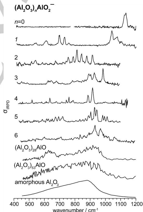
Figure 1. Experimental IRPD spectra of \text{D}_2 -tagged (\text{Al}_2\text{O}_3)_n\text{AlO}_2^- anions compared with the IR-REMPI spectra of neutral \text{AlO}(\text{Al}_2\text{O}_3)_{28.53} and the IR spectrum of amorphous \text{Al}_2\text{O}_3 derived from the optical constants of bulk aluminum oxide for spherical particles in the Rayleigh limit. [5] The n = 0 spectrum is reproduced from ref. [6]. See Fig. S1 and Table S1 for band positions.
