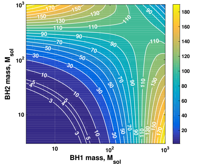
FIG. 5: Improvement in the anticipated event rate for BBH coalescences based on the QNLS (amplitude spectral density) of the proposed scheme as compared to the QNLS (amplitude spectral density) of the equivalent Michelson interferometer.
