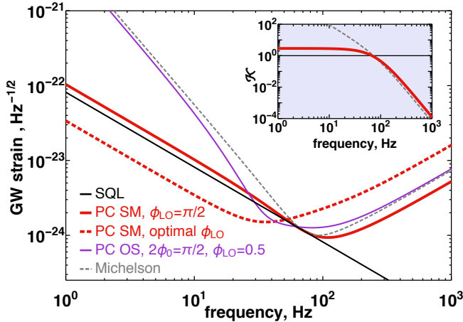
FIG. 3: Quantum noise limited sensitivity (QNLS) of the polarisation circulation (PC) speed meter (red traces) as compared to the QNLS of the equivalent Michelson interferometer (grey dashed trace). Red dashed curve shows the potential of speed meter to beat the free mass SQL (black trace) in a wide band if optimal readout quadrature is measured: \cot \phi_{\text{LO}} = \mathcal{K}_{\text{PCSM}}(0) . In all other cases we assume phase readout, i.e. \phi_{\text{LO}} = \pi/2 . Purple trace represents the QNLS of proposed scheme in a special regime ( 2\phi_0 = \pi/2 ) where an optical spring is created due to transfer of signal from phase to amplitude quadrature in the polarisation circulator. Hereafter we assume mirrors mass M = 200 kg, power, circulating in each arm P_c = 3 MW, laser wavelength \lambda_0 = 2 \mu\text{m} and effective interferometer bandwidth \gamma/2\pi = 80 Hz.
