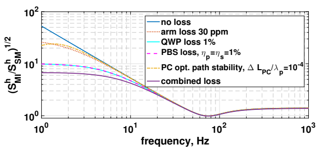
FIG. 4: Influence of different sources of loss and imperfection on quantum noise-limited sensitivity of the polarisation circulation speed meter as compared to the equivalent Michelson interferometer.
