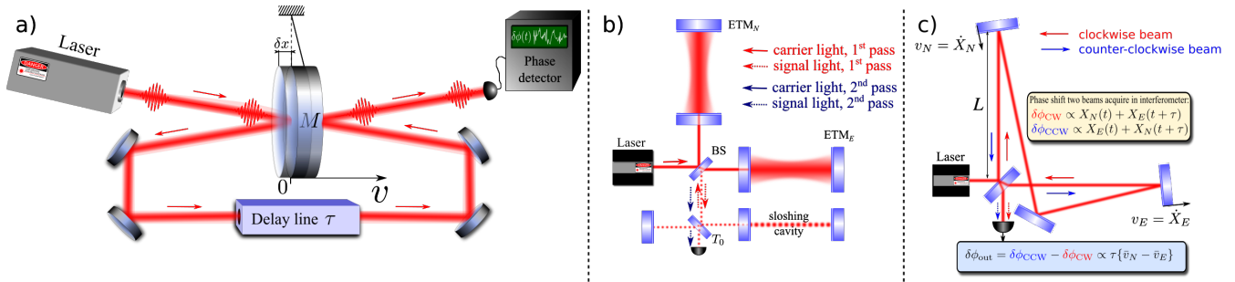
FIG. 1: a) Conceptual scheme of speed measurement (a) and two variants of its implementation in laser interferometers, (b) as sloshing speed meter, and (c) as Sagnac speed meter.
