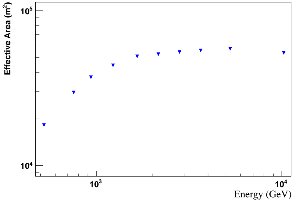
Figure 5.19: The effective area of each energy bin, used in the calculation of the cosmic electron spectrum.
