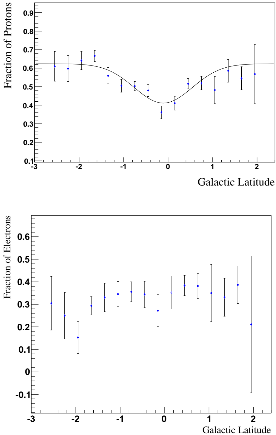
Figure 5.13: Estimated proton (top) and electron (bottom) fractions with Galactic latitude. All profiles included events in the longitude range of -20 < l < 16^\circ and 19 < l < 30^\circ .
