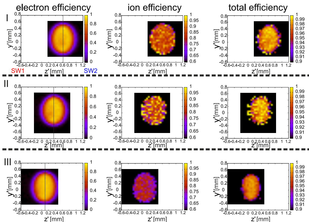
Figure 4.7.: 2-dimensional map of the detection efficiencies of the CEMs under variation of the voltage configuration at the sidewalls (SW1, SW2) of the vacuum chamber, i.e shift of the electric potential along the quantization axis. For voltage settings see table 4.3.
