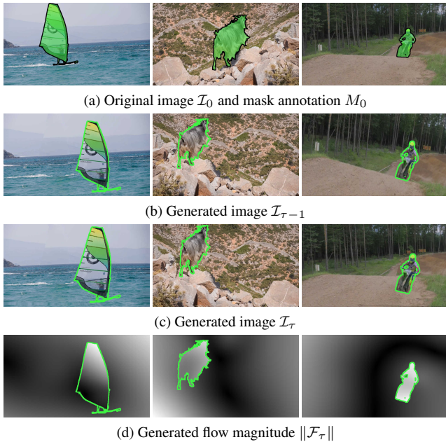
Figure 4: Lucid data dreaming examples. From one annotated frame we generate pairs of images ( \mathcal{I}_{\tau-1} , \mathcal{I}_{\tau} ) that are plausible future video frames, with known optical flow ( \mathcal{F}_{\tau} ) and masks (green boundaries). Note the inpainted background and foreground/background deformations.
