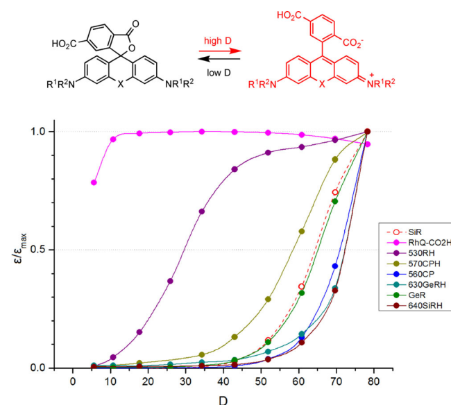
Figure 2. Normalized extinction \epsilon/\epsilon_{\text{max}} at \lambda_{\text{max}} of the dyes from Table 1 versus dielectric constant D of dioxane–water mixtures ( 575RH and 6-ROX are unresponsive and are not included). The D 0.5 values correspond to the intersection of interpolated graphs with \epsilon/\epsilon_{\text{max}} = 0.5 line. [1a]
