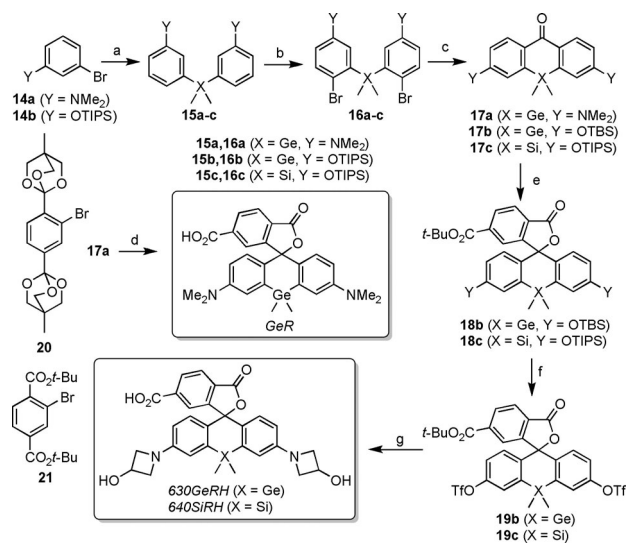
Scheme 2. Synthesis of GeR and SiR dyes. a) n\text{BuLi} , -78 °C, then Me 2 GeCl 2 or Me 2 SiCl 2 ; b) NBS; c) n\text{BuLi} or t\text{BuLi} , -78 °C, then Me 2 NCOCl; d) 20 , t\text{BuLi} (2 equiv), -78 °C to RT, then HCl; e) 21 , n\text{BuLi} , THF-pentane, -100 °C to RT; f) TBAF, then Tf 2 O, pyridine; g) 3-( tert -butylsilyloxy)azetidone, cat. Pd 2 (dba) 3 /XPhos, K 2 CO 3 , dioxane, 100 °C, then TBAF, then TFA.
