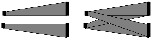
Figure 2: Reachpipe Completion (i) R(t) ; (ii) [R](t)
