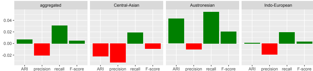
Figure 5: Evaluation results (difference between performance of our method and baseline). Green bars indicate positive values (our method outperforms baseline) and red bars indicate negative values.
