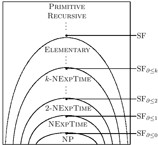
Figure 1: The subfragments of SF scale over the major nondeterministic complexity classes in \text{ELEMENTARY} , while SF itself goes even beyond.
