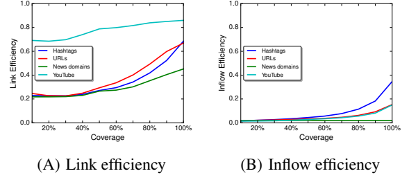
Figure 7: The average link and in-flow efficiencies versus the percentage of covered memes.
