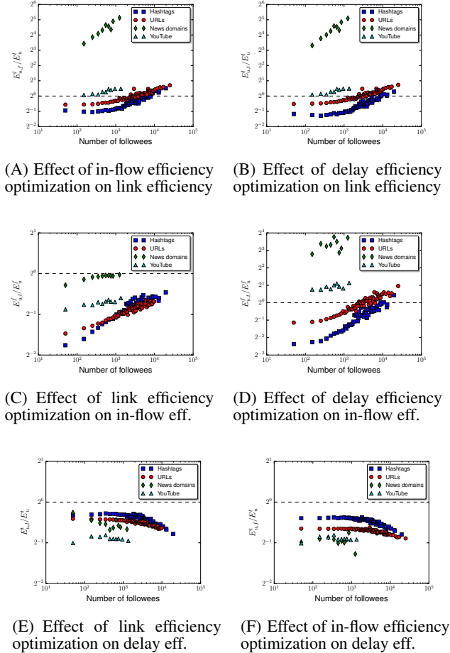
Figure 10: The effect of optimization of one of the efficiencies on another efficiency, plotted as the ratio of the efficiency in the optimized network and the original network against the number of followees. The dashed line marks the ratio equal to 1, which corresponds to the lack of change in the efficiency due to the respective optimization.
