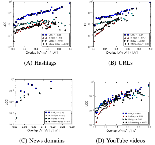
Figure 15: Local clustering coefficient of the optimized ego-networks versus the overlap between the original ego-network and the ego-networks optimized for link (blue squares), in-flow (red triangles), delay (teal triangles), and inflow-delay efficiency (black triangles).
