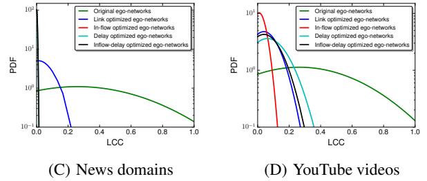
Figure 13: The distributions of local clustering coefficient (LCC) of the original ego-network (green circles) and the ego-networks optimized for link (blue circles), in-flow (red circles), delay (teal circles), and inflow-delay efficiency (black circles) for: (A) hashtags, (B) URLs, (C) news domains, (D) and YouTube videos.
