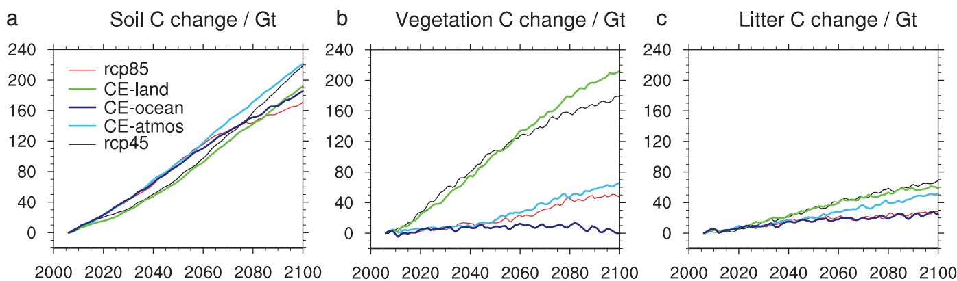
Figure 5. Total global annual mean carbon content change in the (a) soil, (b) vegetation, and (c) litter pools in experiments rcp85, CE-land, CE-ocean, CE-atmos, and rcp45 for the years 2006–2100.
