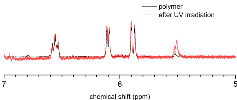
Figure 26. Zoom in on ^1\text{H} NMR spectra of nanocontainers before and after UV irradiation.
