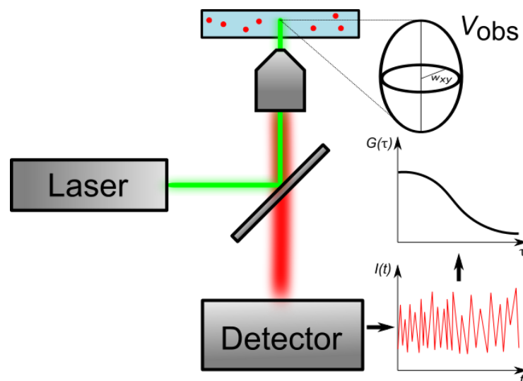
Figure 28. FCS Setup. V_{\text{obs}} is the observation volume.
