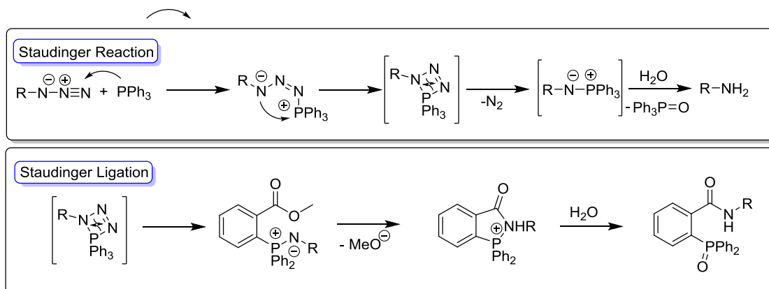
Scheme 2. Mechanisms of the Staudinger Reaction and the Staudinger Ligation.
