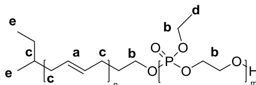
Figure 70. Poly(butadiene)- b -poly(ethyl ethylene phosphate).
