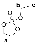
Figure 68. Ethyl ethylene phosphate
