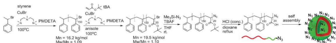
Scheme 4. Strategy for azide-functionalised polymersomes. Reproduced from [88] with permission of The Royal Society of Chemistry.
