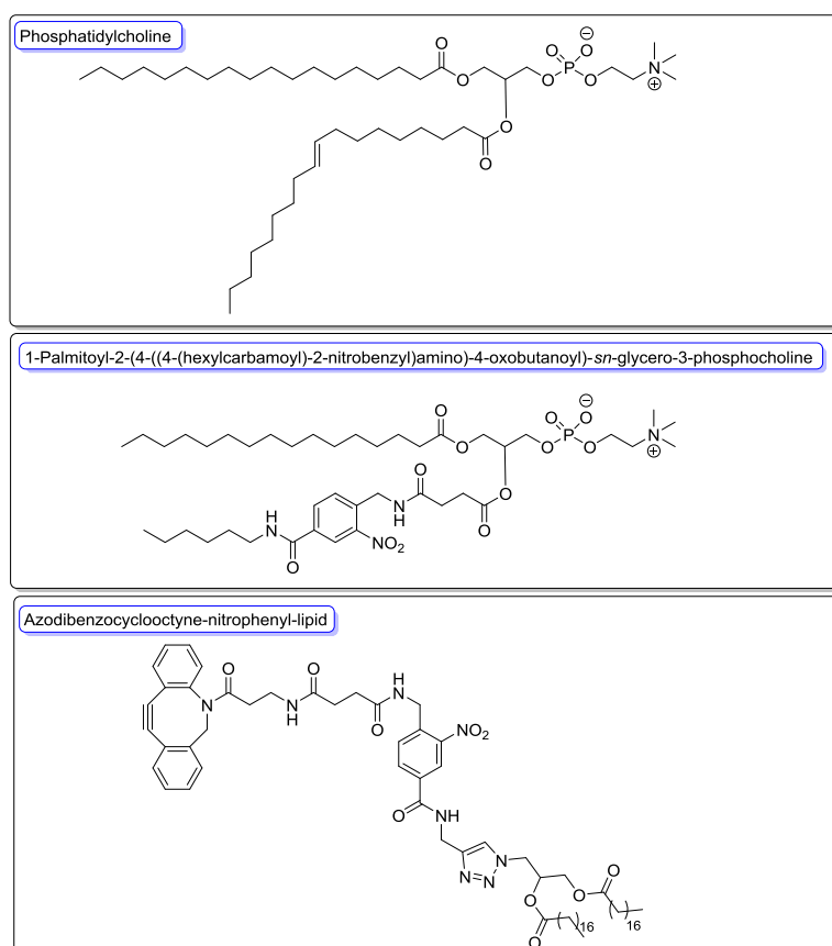
Scheme 3. Structure of phosphatidylcholine (top), its synthetic analogue 1-palmitoyl-2-((4-((hexylcarbamoyl)-2-nitrobenzyl)amino)-4-oxobutanoyl)-sn-glycero-3-phosphocholine (middle) and the synthetic lipid azodibenzocyclooctyne-nitrophenyl-lipid (bottom).
