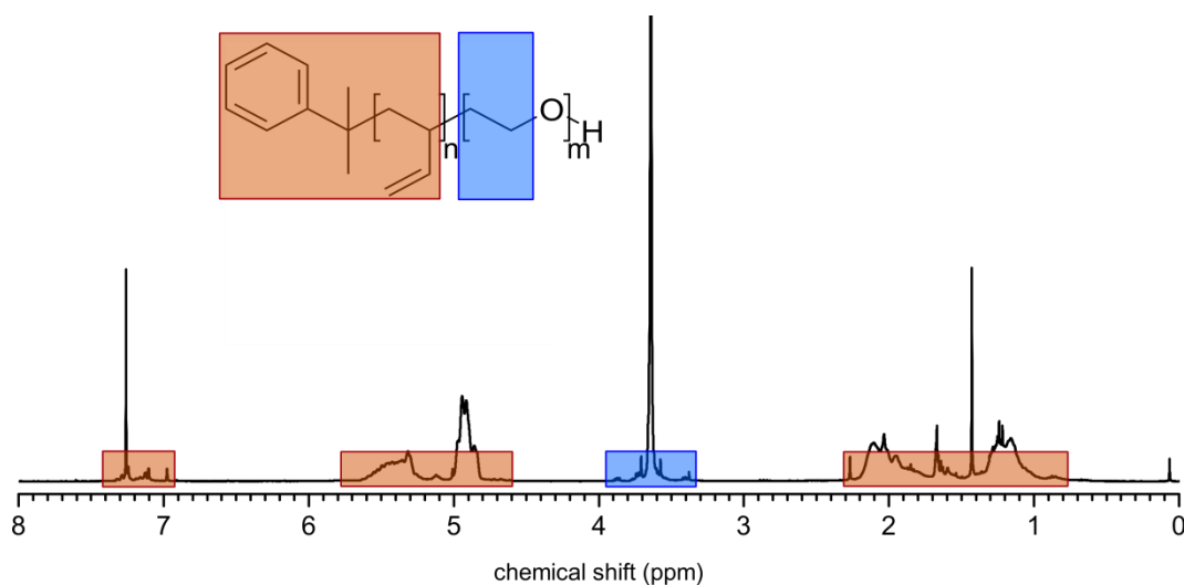
Figure 31. ^1\text{H} NMR (300 MHz, 298 K) spectrum of \text{PB}_{85}\text{-}b\text{-PEO}_{68} in \text{CDCl}_3 .
