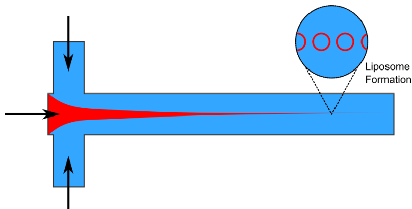
Figure 8. Illustration of microfluidic hydrodynamic focusing. The cross junction is shown. The central channel is filled with a lipid solution in alcohol (red). At the junction, two water channels (blue) focus the central stream.
