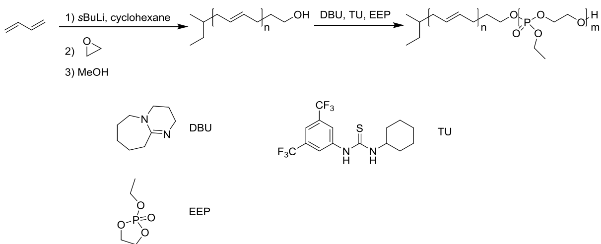
Scheme 12. Synthetic protocol for poly(butadiene)- block -poly(ethyl ethylene phosphate) block copolymers. For clarity only the 1,4-addition of 1,3-butadiene is shown.
