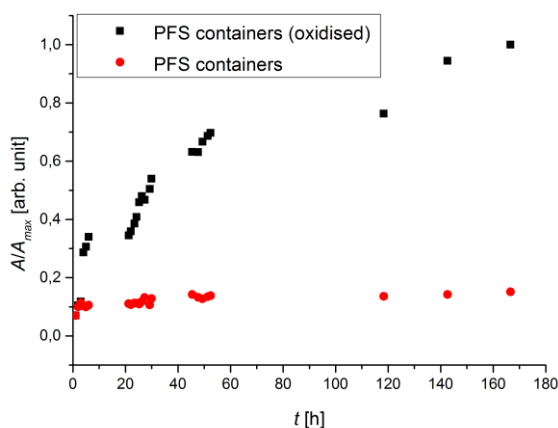
Figure 24. Release of 2-propylpyridine from PFS nanocontainers over time (red) and upon enzymatic oxidation with glucose oxidase in the presence of glucose (black).
