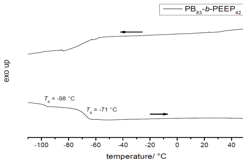
Figure 55. DSC curve of PB 83 - b -PEEP 42 (cooling and 2nd heating curve, 10\text{K}\cdot\text{min}^{-1} ). T_g is the glass transition temperature.
