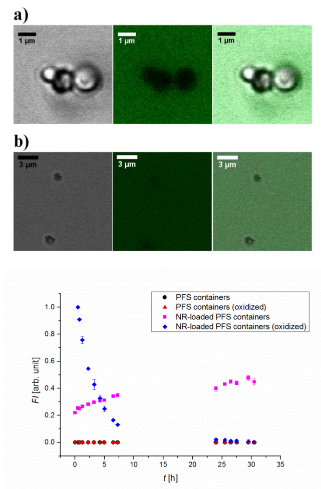
Figure 23. Confocal laser scanning microscopy (CLSM) images of PFS nanocontainers dispersed in FITC-dextran before (a) and after (b) oxidation with H_2O_2 . Images show the transmission channel (left), fluorescent channel (middle) and the overlay (right). c) Fluorescence intensity over time of PFS nanocontainers (black spheres), PFS nanocontainers with H_2O_2 (red triangles), Nile Red-loaded PFS nanocontainers (pink squares) and Nile Red-loaded PFS nanocontainers with H_2O_2 (blue diamonds). Error bars represent the mean of two separate measurements.
