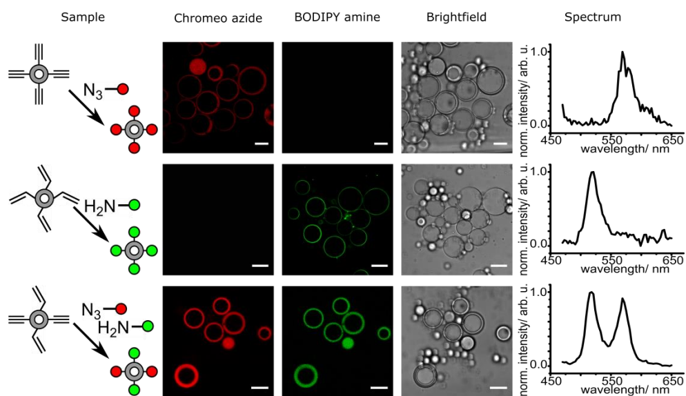
Figure 40. CLSM results for orthogonally labeled polymersomes. Shown are the chromeo azide channel (red), the BODIPY amine channel (green) and the brightfield channel. The scale bars are 30 \mu\text{m} . A spectrum of the fluorescent intensity was taken to identify the dyes.
