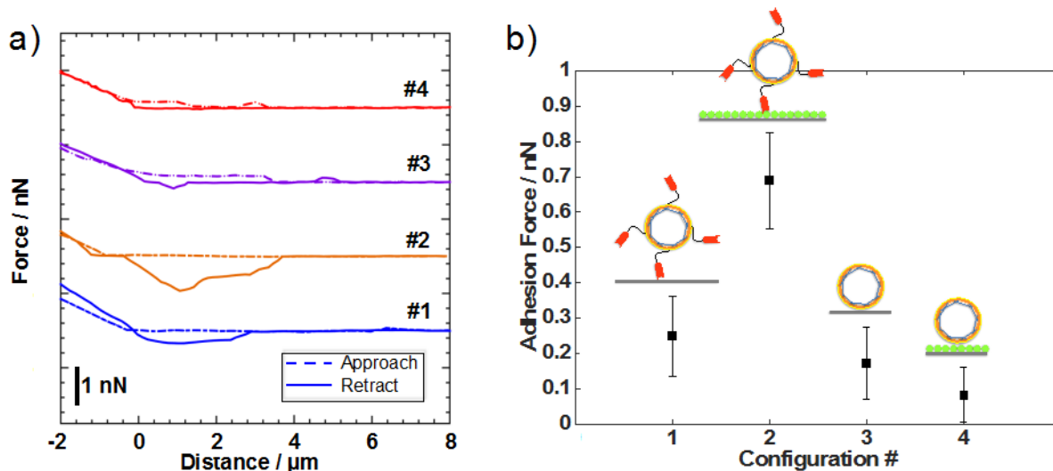
Figure 46. Force-distance curves of biotin-functionalised and non-functionalised vesicles on NeutrAvidin-coated glass and glass (a). Dashed lines are the approach, solid lines the retract. Mean adhesion force of biotin-functionalised and non-functionalised vesicles on glass and NeutrAvidin-coated glass (b).
