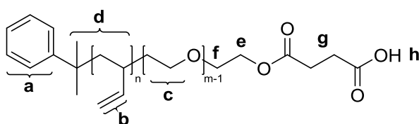
Figure 65. Poly(butadiene)- block -poly(ethylene oxide) with an acrylate end group functionalisation
