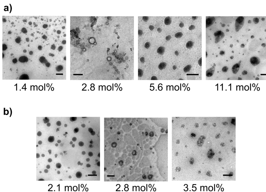
Figure 48. TEM micrographs of PB_{85} - b - PEO_{68} samples crosslinked with V-65 (a and b). The amount of V-65 relative to the PB double bonds is given below each image. Scale bars are 200 nm, with the exception of both 2.8 mol% images (100 nm) and the 3.5 mol% image (400 nm).
