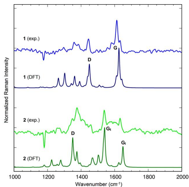
Figure 3. Experimental and DFT-simulated Raman spectra of 1 (light and dark blue) and 2 (light and dark green). G_t and G_l are the G modes of 2 occurring along the transversal and longitudinal axes of the molecule. The G mode of 1 is longitudinal.
