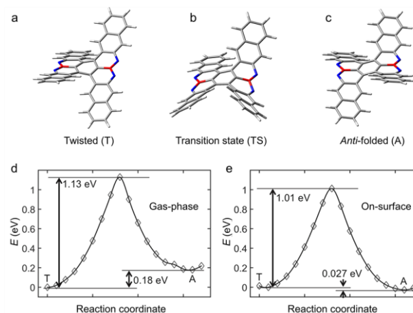
Figure 1. (a-c) DFT-optimized molecular geometries of the twisted and anti -folded 2 and the transition state from T to A. (d) Gas-phase and (e) on-surface energy barriers for the transformation from T to A calculated by the nudged-elastic-band (NEB) method.
