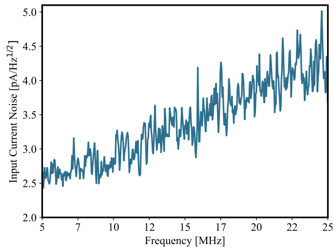
Fig. 5. Input noise density \bar{i}_{en} for a single channel measured using cold redundancy (only one PRF). The requirement for GRACE-FO in this configuration is 5 \text{ pA/Hz}^{1/2} at 16 MHz. The value obtained is around 3.5 \text{ pA/Hz}^{1/2} , fulfilling the requirement. The measurement was repeated for all channels of all PRFs obtaining similar results.
