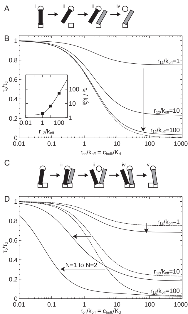
Figure 4. Effect of multiple binding sites on stability under competition. The exchange time ( \tau_e ) is normalized to the dissociation time under dilution ( \tau_d ), and is shown as a function of the binding rate of competitors from solution relative to the unbinding rate ( r_{\text{on}}/k_{\text{off}} ) or, equivalently, the bulk concentration of competitors over the dissociation constant ( c_{\text{bulk}}/K_d ). (A) Schematic illustrating the exchange mechanism available in the case of a single primary binding site. (gray) competing molecule. Naturally, the same process can take place on the secondary binding site. (B) Exchange time with one primary binding site ( N = 1 ). Arrow shows direction of increased stability under dilution ( r_{12}/k_{\text{off}} ). Results calculated using Equations (4) and (6). (Dotted line) Approximation valid for a complex very stable against dilution (large r_{12}/k_{\text{off}} ), calculated from Equation (7). (Inset) Dissociation time under dilution duplicated from Figure 3B. Symbols indicate parameters (values of r_{12}/k_{\text{off}} ) considered in the main graph. (C) Schematic illustrating the novel mechanism present with several primary binding sites ( N > 1 ). (D) Exchange time with two primary binding sites ( N = 2 ). (Solid lines) Two primary binding sites. (Dashed lines) Results for one primary binding site duplicated from panel B; arrows indicate change from one to two sites. Results for N = 2 calculated using SD Equation (S13–S15).
