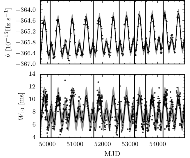
Figure 12. Comparison between the MPE \Delta\epsilon_p -model with N = 6 jumps (solid line) and the observed spin-down and beam-width data (black dots). Vertical lines mark the times of the six (positive) jumps in \epsilon_p(t) . The shaded region indicates the estimated 1\sigma noise level.
